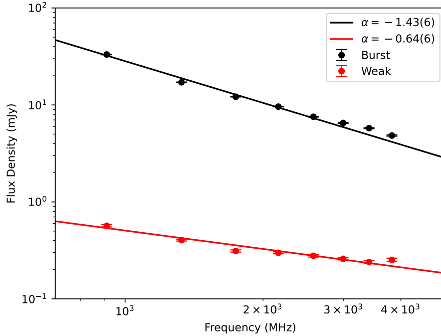
Figure 7. The flux densities of the burst (black dots) and weak (red dots) modes. The solid lines represent the fitting results using the power-law model.
