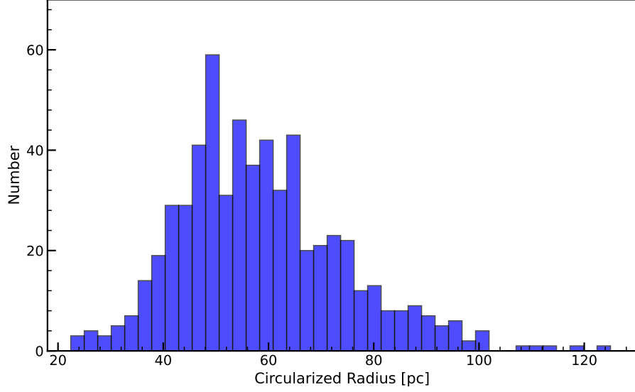
Figure 5. Histogram of circularized radius for 609 H II regions in NGC 628.
