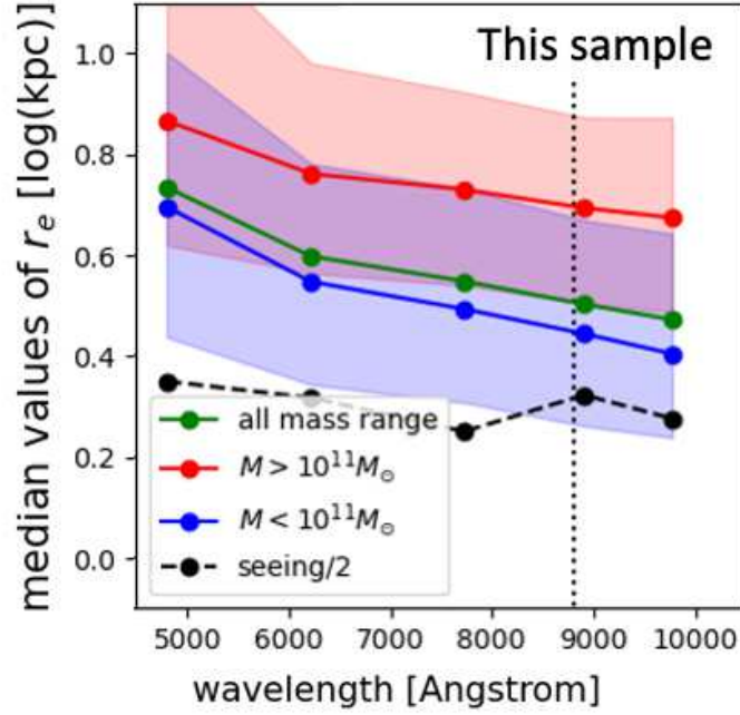
Figure 3. The measured r_e values in the five HSC bands ( grizy ) for our massive quiescent galaxy sample. The colored data points are the median value of r_e in each band and for the three mass bins: red for high mass bin ( M_* > 10^{11} M_\odot ), blue low mass bin ( M < 10^{11} M_\odot ), and green for the full sample. The black points represent half values of the average seeing sizes in each band. The red and blue shades illustrate the range (25%–75%) of the sample in the two mass bins.
