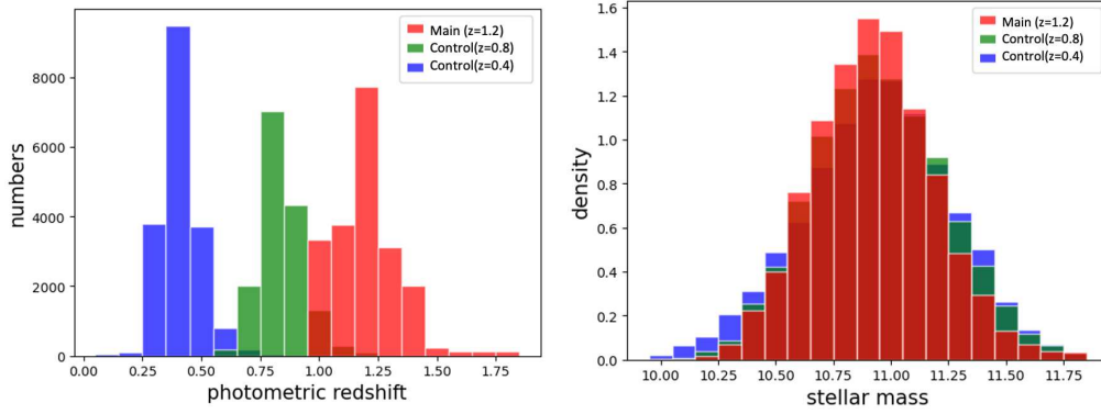
Figure 1. The photometric redshift and stellar mass distribution for our massive quiescent galaxy sample at z \sim 1.2 (red) and the two control samples at lower redshift (blue for z \sim 0.4 and green for z \sim 0.8 ).
