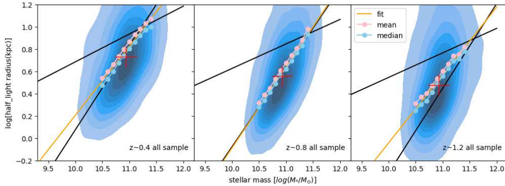
Figure 8. The size–mass relation for massive quiescent galaxies for our main sample at z = 1.2 , and two control samples at z \sim 0.8 and z \sim 0.4 . The blue contour shows the number density of the three samples, each contains 18k–19k objects, while the pink and blue circles represent the mean and median values of our samples respectively. The solid red crosses represent the median values of r_e and M_* at each redshift bin. The reference black solid lines are from van der Wel et al. (2014) for ETGs and LTGs. The orange lines show our best fitting results (minimum \chi^2 ).
