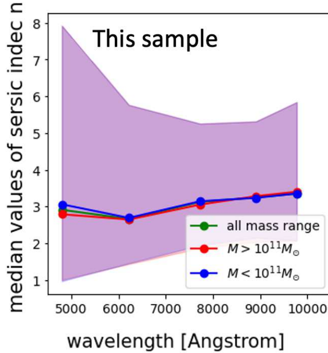
Figure 4. The value and range of the Sérsic index n in the five HSC bands for our massive quiescent galaxy sample. Color codes and shades for the data are the same as in Figure 3.
