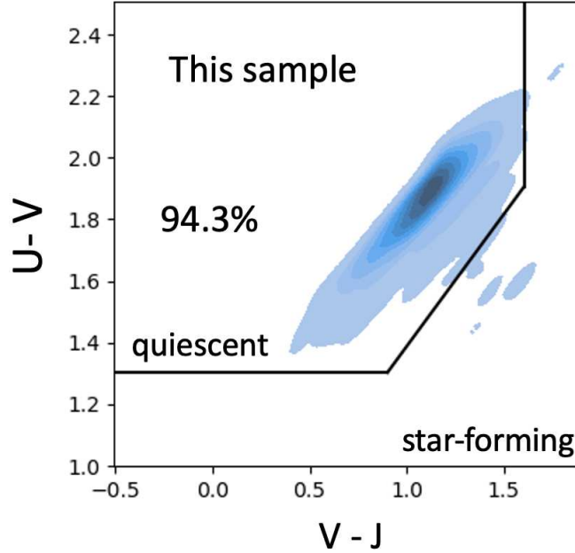
Figure 2. Distribution of our z \sim 1.2 sample in the rest-frame UVJ diagram. The vast majority of our color-selected massive galaxies lie in the quiescent region of the UVJ diagram (Williams et al. 2009).
