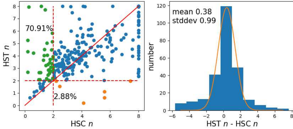
Figure 6. Comparison of Sérsic index n between HSC and HST images (left) and their difference histogram ( \Delta n = n_{\text{HST}} - n_{\text{HSC}} , right). The red solid line in the left panel marks the 1:1 ratio, while the red dashed lines are the separation of disk-like and bulge-like galaxies at n = 2.0 . Galaxies that experience a type swap (i.e., disk-like in one and bulge-like in another image) are colored in green and orange. The mean and \sigma for \Delta n is 0.38 \pm 0.99 , suggesting significant differences.
