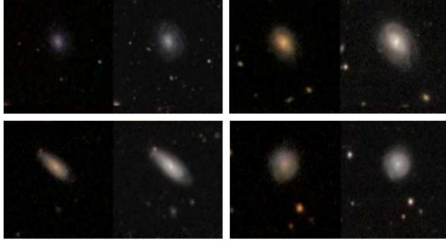
Figure 1. Differences in depth and resolution between GZ2 and DECaLS images, with GZ2 on the left and DECaLS on the right.
