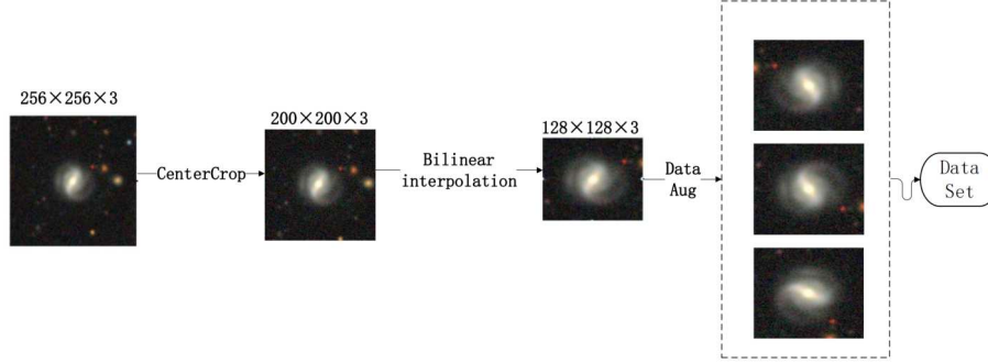
Figure 4. The process of preprocessing in the training set. The samples in the training set, whether from the Galaxy10decals data set or the GZD-5 project, all need to repeat the above steps, only with different processing details.
