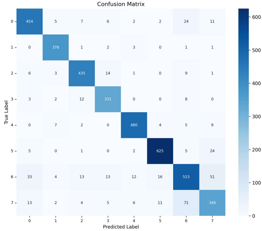
Figure 9. The misclassification matrix of the model for the test data set.
