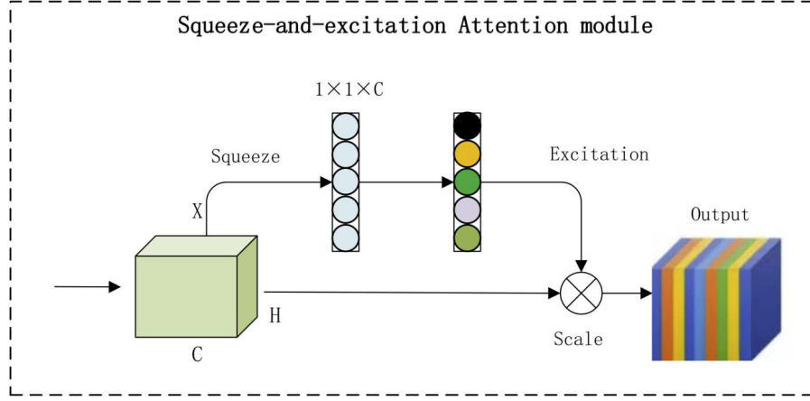
Figure 6. Squeeze-and-excitation Attention module's structure.
