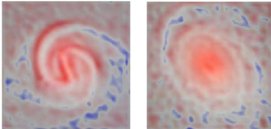
Figure 17. The color mapping and position mapping in the figure of the changes in the channel activation degrees of the model for the data of two spiral galaxies.
