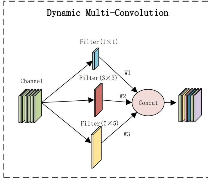
Figure 7. Dynamic Multi-conv module's structure.
