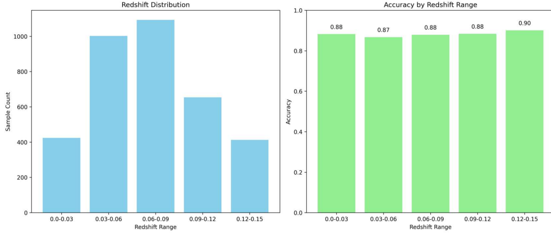
Figure 15. The distribution of redshift values in the test set and the response of the algorithm within different redshift intervals of this data set.
