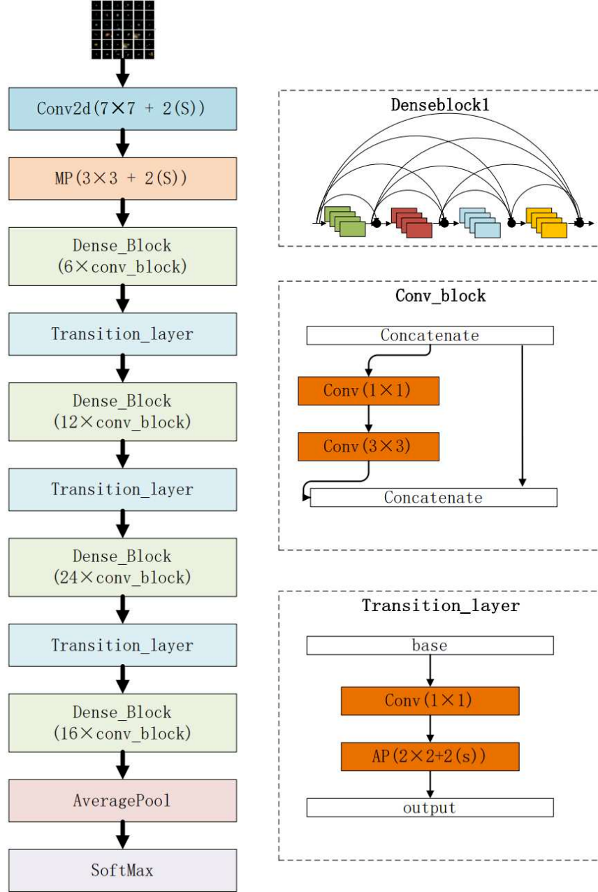
Figure 5. The architecture of DenseNet-121.
