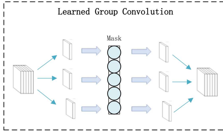
Figure 8. Learned Group-conv module's structure.
