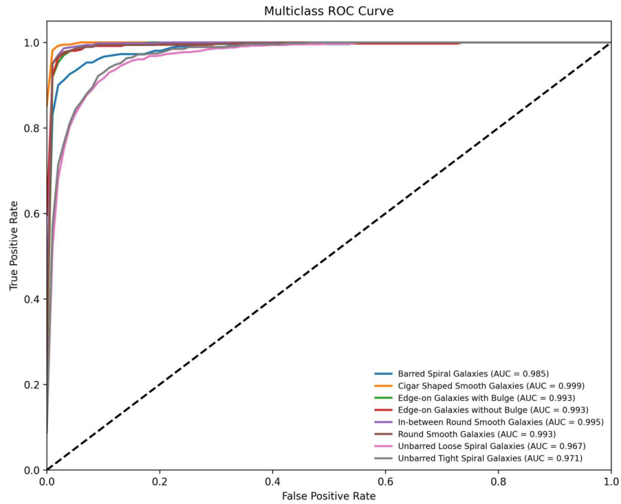
Figure 10. The ROC curves of the DenseNet-SE4 model.
