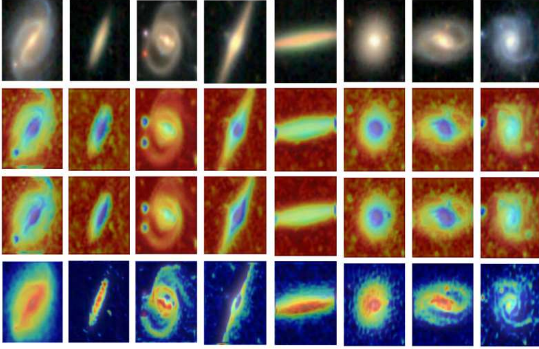
Figure 18. Visualization diagrams of the eight categories are presented. The images in the first row are the input images, those in the second row are before the addition of the attention mechanism, the ones in the third row are after the addition, and the pictures in the fourth row are the Grad-CAM diagrams.
