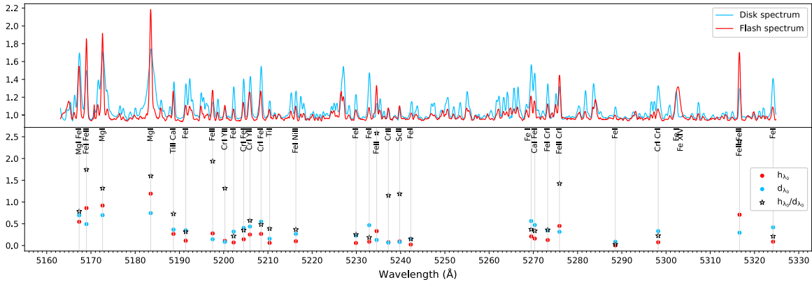
Figure 6. Top panel: 1D flash spectrum (red) superposed with the inverted on-disk absorption spectrum (blue) for contrast. Bottom panel: The measured values of relative line height ( h_{\lambda_0} ) in red and depth ( d_{\lambda_0} ) in blue, as well as their ratio ( h_{\lambda_0}/d_{\lambda_0} ) in black presented for distinct spectral lines.
