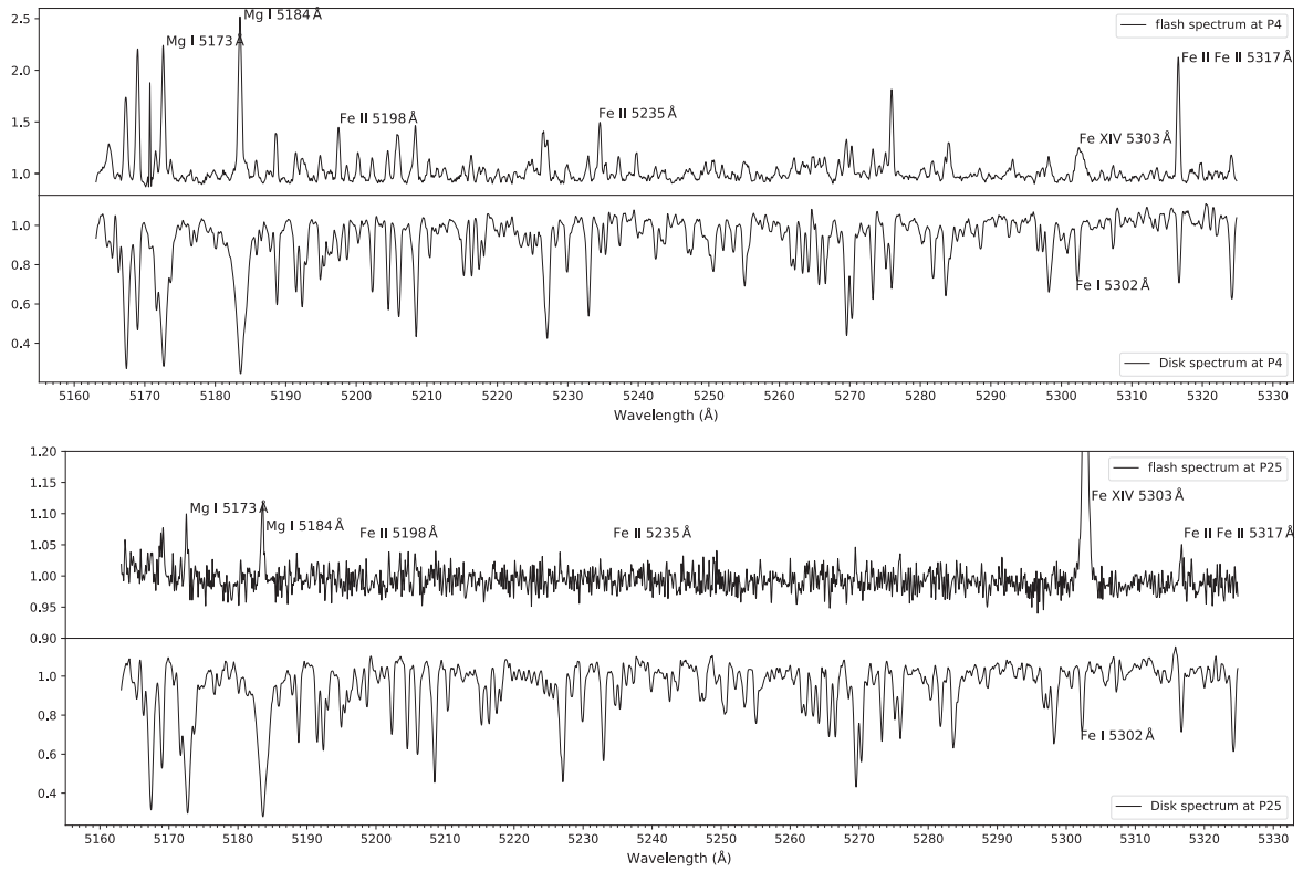
Figure 4. Sample one-dimensional spectra at a specific spatial pixel P4 and P25. Upper panel: the flash spectrum and the corresponding disk spectrum at P4; lower panel: the flash spectrum and the corresponding disk spectrum at P25. All spectra are normalized with respect to their continuum levels.
