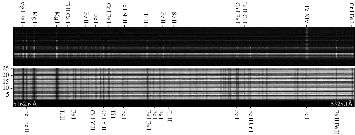
Figure 2. Raw flash spectrum data (top) and solar spectrum data (bottom). In each frame: The X-axis represents the dispersion direction, covering a wavelength range of approximately 5162.60–5325.08 Å; while the Y-axis corresponds to the slit direction. Key spectral lines, identified after wavelength calibration, are marked.
