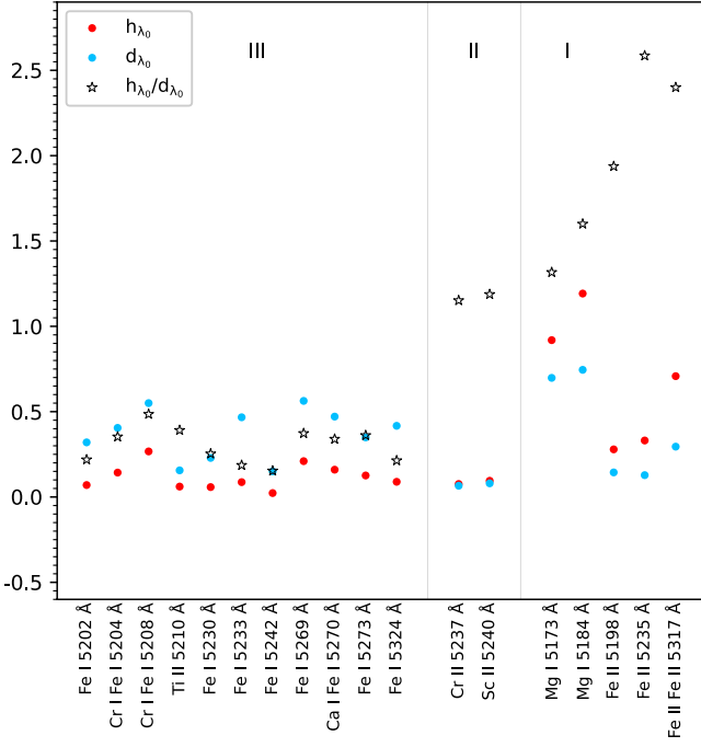
Figure 7. A figure showing the spectral parameters h_{\lambda_0} , d_{\lambda_0} and their ratio h_{\lambda_0}/d_{\lambda_0} for spectral lines, categorized by formation layers as summarized in Table 1. Categories: I. Low chromosphere, II. Upper photosphere (FIP atoms), III. Upper photosphere (neutral atoms).
