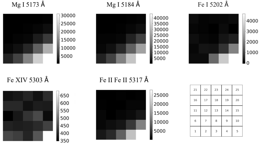
Figure 3. Two-dimensional reconstructed images centered on selected flash emission lines and coronal line Fe XIV 5303 Å. The bottom-right panel illustrates the spatial pixel correspondence to the slit direction, which is labeled on the Y-axis in the raw data (Figure 2).
