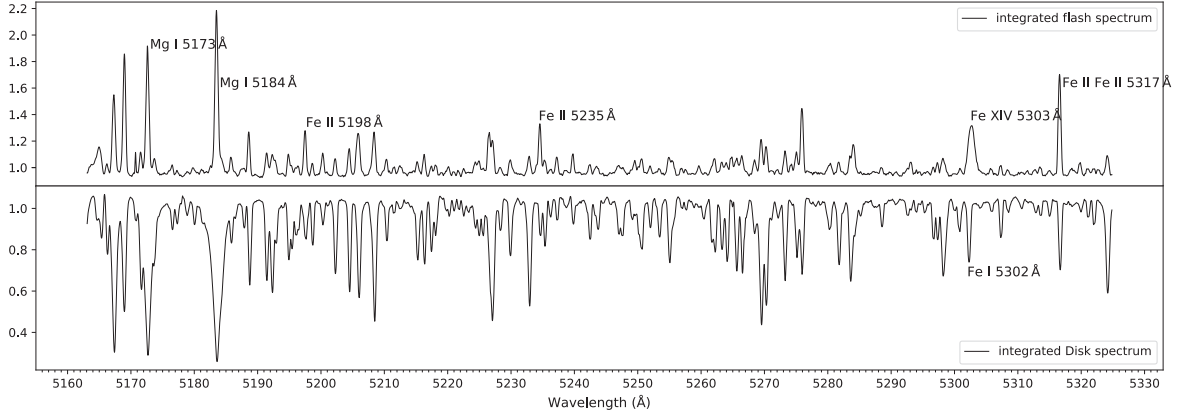
Figure 5. Integrated one-dimensional spectra. Upper panel: the flash spectrum; lower panel: the disk spectrum. Both spectra are normalized to their respective continuum levels for direct comparison.
