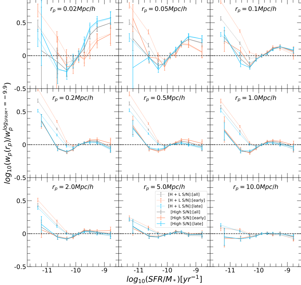
Figure 4. Normalized w_p(r_p) from SDSS, measured at different r_p (as indicated) as a function of sSFR, for the high-S/N SFG sample (solid lines) and the sample additionally including low-S/N SFGs (dotted lines). The gray, orange, and cyan symbols/lines correspond to the results obtained using the full reference sample and the reference samples with only early-type or late-type galaxies, respectively.
