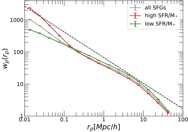
Figure 5. Projected 2PCFs between star-forming galaxies and the reference galaxy sample from TNG300. The gray symbols/lines represent the full sample of star-forming galaxies, while the red and green symbols/lines correspond to the subsamples of high- and low-sSFR galaxies, respectively. The dashed line shows the real-space correlation function of \xi(r) = (r/5 h^{-1} \text{Mpc})^{-1.8} as a reference.
