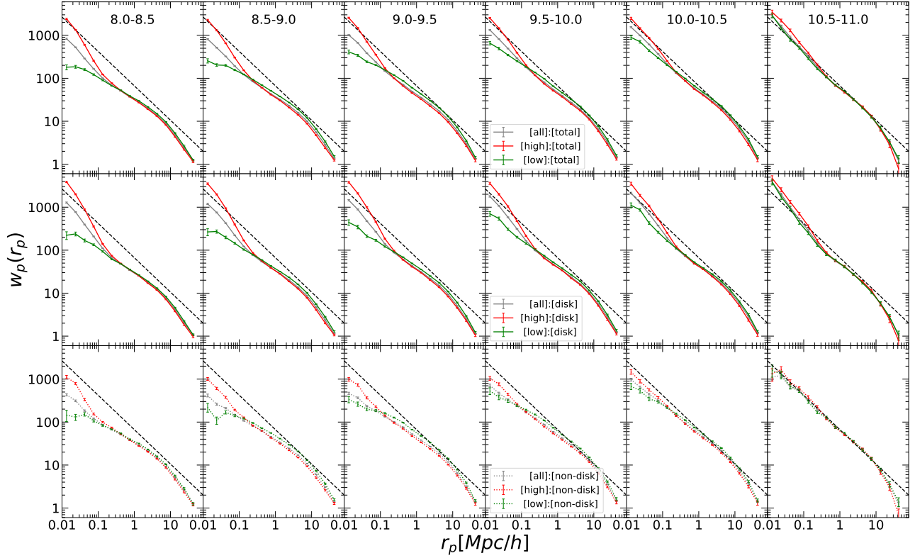
Figure 6. The projected 2PCFs of star-forming galaxies (SFGs) from TNG300, measured for SFGs in different stellar mass intervals, as indicated. In each panel, the gray, red, and green symbols/lines represent the full sample of SFGs and the two subsamples of high- and low-sSFR galaxies, respectively. The top panels show results based on the full reference sample, while the middle and bottom panels correspond to reference samples including only disk galaxies or non-disk galaxies, respectively.
