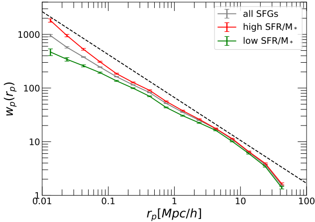
Figure 1. Projected 2PCCFs between star-forming galaxies and the reference galaxy sample from SDSS. The gray symbols/lines represent the full sample of star-forming galaxies, while the red and green symbols/lines correspond to the subsamples of high- and low-sSFR galaxies, respectively. The dashed line shows the real-space correlation function of \xi(r) = (r/5 h^{-1} \text{Mpc})^{-1.8} as a reference.
