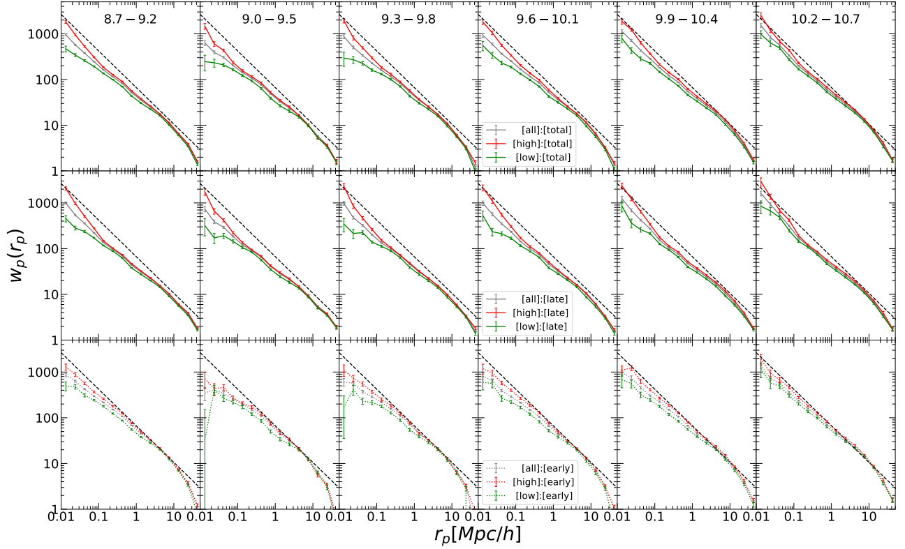
Figure 2. The projected 2PCCFs of star-forming galaxies (SFGs) from SDSS, measured for SFGs in different stellar mass intervals, as indicated. In each panel, the gray, red, and green symbols/lines represent the full sample of SFGs and the two subsamples of high- and low-sSFR galaxies, respectively. The top panels show results based on the full reference sample, while the middle and bottom panels correspond to reference galaxies of late-type and early-type morphology, respectively.
