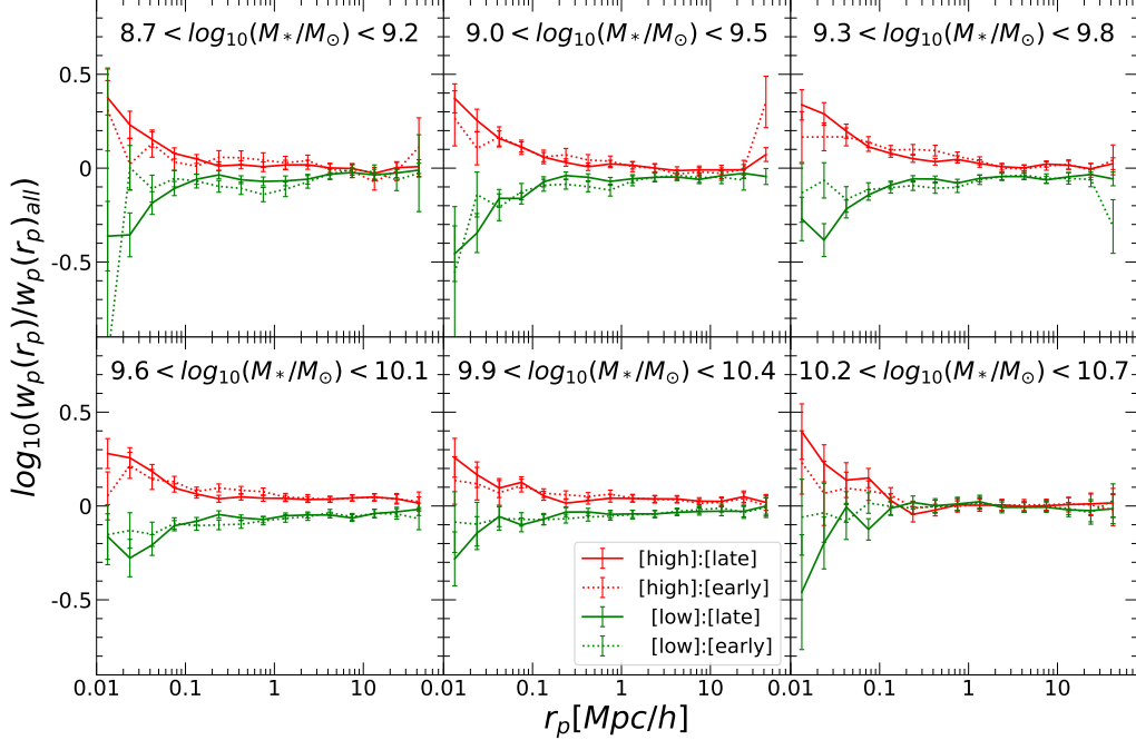
Figure 3. Ratio of the w_p(r_p) measured for the high-sSFR (red) and low-sSFR (green) subsamples relative to that of the full SFG sample as a function of projected separation r_p , measured from SDSS. In each panel, the dashed and solid symbols/lines represent the results obtained using reference samples of early-type and late-type morphology, respectively.
