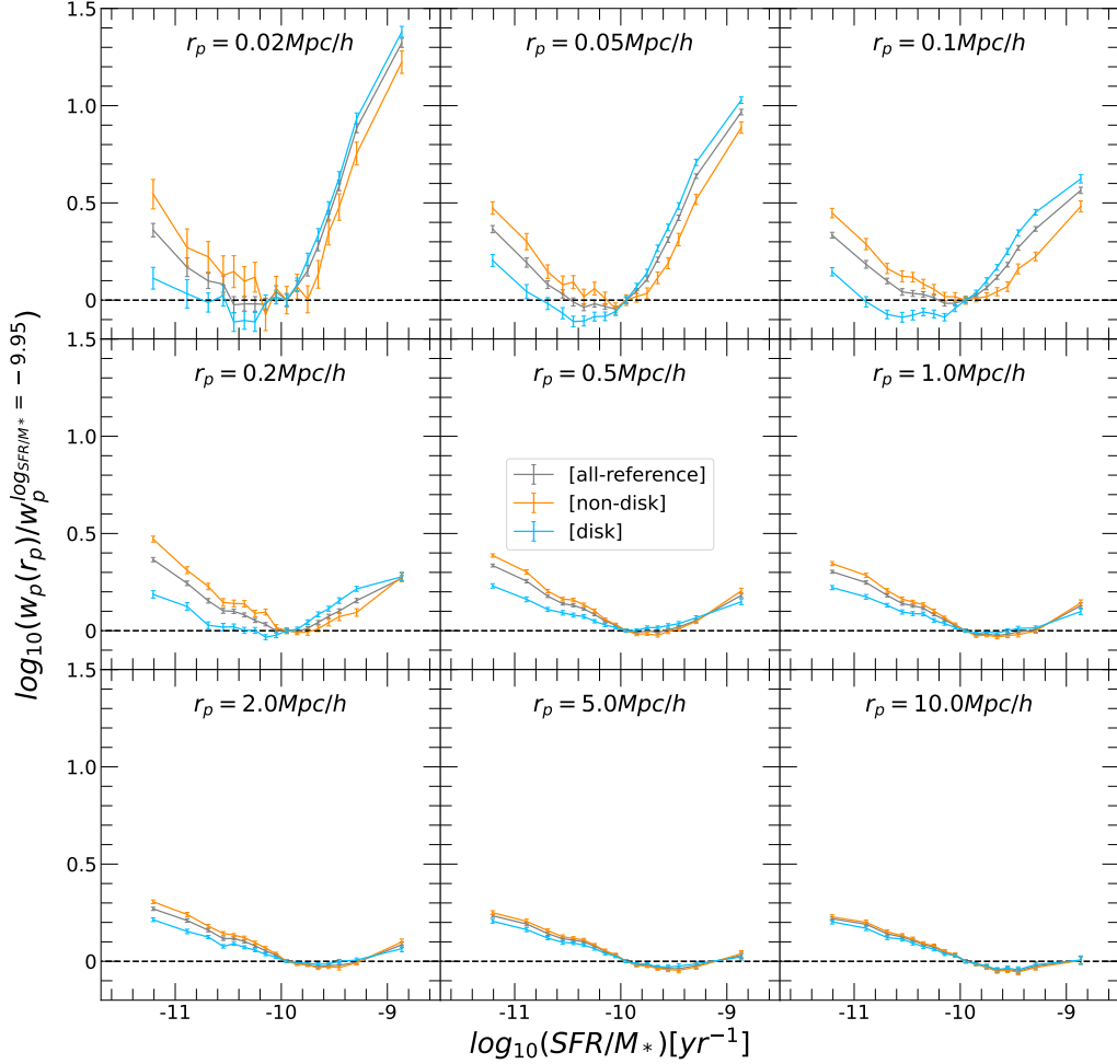
Figure 8. Normalized w_p(r_p) from TNG300, measured at different r_p (as indicated) as a function of sSFR, for the high-S/N SFG sample (solid lines) and the sample additionally including low-S/N SFGs (dotted lines). The gray, orange, and cyan symbols/lines correspond to the results obtained using the full reference sample and the reference samples with only non-disk galaxies or disk galaxies, respectively.
