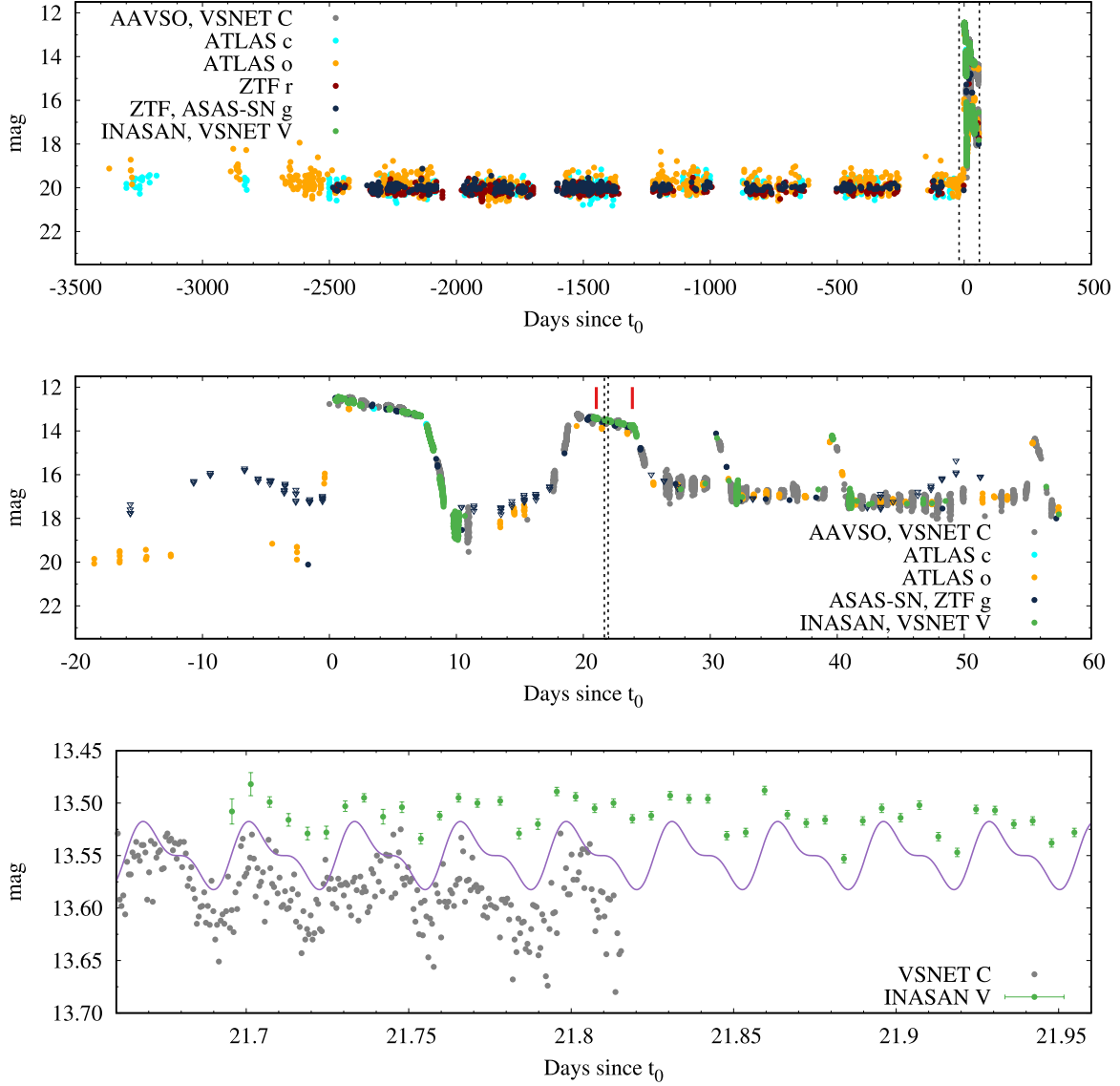
Figure 1. The lightcurve of J0722 combining V -band photometry from INASAN Terskol and Kislovodsk telescopes (Section 2.4) with V -band and unfiltered CV -band measurements collected by VSNET and AAVSO observers (including CV photometry from the two NMW cameras), ASAS-SN g , ATLAS o (orange) and c (cyan), and ZTF g and r data. The top panel shows the complete combined lightcurve with the vertical dashed lines indicating the outburst plotted in the middle panel. The vertical dashed lines in the middle panel indicate time range of the bottom plot that presents an example section of the lightcurve where superhumps are visible (Section 3.2). The purple curve approximates the superhump shape as a sum of two sine waves, one with a period from Equation (3) and the peak-to-middle amplitude of 0.025 mag and the other with twice that period and half the amplitude (see Figure 4), it is plotted to guide the eye. The outburst plot (middle panel) includes ASAS-SN g upper limits (triangles) along with the positive detections (filled circles). Vertical red bars mark the times of spectroscopic observations described in Section 2.3.
