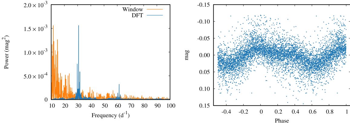
Figure 4. Power spectrum with its corresponding spectral window (left panel) and phased lightcurve of J0722 (right panel) during the rebrightening constructed by combining INASAN-Kislovodsk BVR and VSNET Clear band data. This data set combines the data presented in the middle and lower panels of Figure 3 with additional Clear band photometry. The lightcurve (right panel) is phased with the light elements HJD(TT) = 2460721.0757 + 0.032546 \times E corresponding to the highest peak in the rebrightening power spectrum (left panel).
