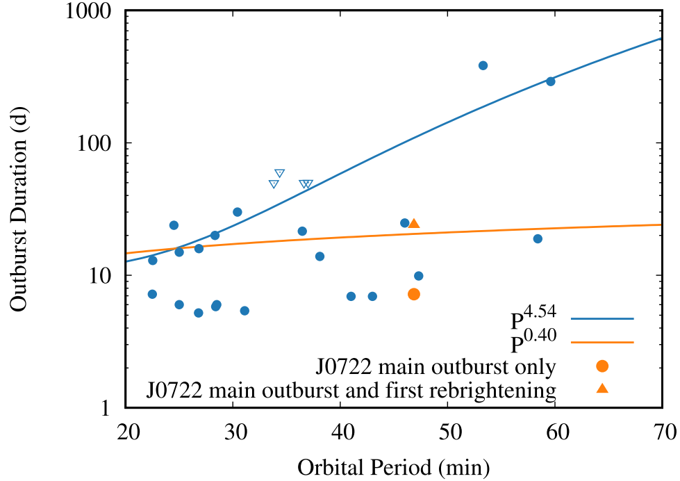
Figure 5. Outburst duration as a function of the orbital period for AM CVn stars from Cannizzo & Ramsay (2019), Pichardo Marciano et al. (2021), Rivera Sandoval et al. (2022), Painter et al. (2024). For systems where Cannizzo & Ramsay (2019) and Pichardo Marciano et al. (2021) give different outburst durations (KL Dra, CP Eri) both estimates are plotted as they are presumably based on different outbursts. Open triangles represent upper limits on the outburst duration. The top blue curve represents the empirical relation of Levitan et al. (2015). The bottom orange curve is the accretion disk limit cycle model of Cannizzo & Nelemans (2015), Cannizzo & Ramsay (2019).
