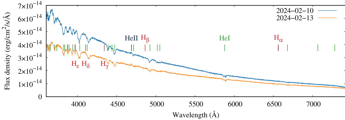
Figure 2. The spectra of J0722 obtained with the 2.5 m SAI MSU telescope during the rebrightening. The green and dark blue marks show the locations of prominent He I and He II lines, respectively. The red marks indicate the expected location of Balmer lines.
