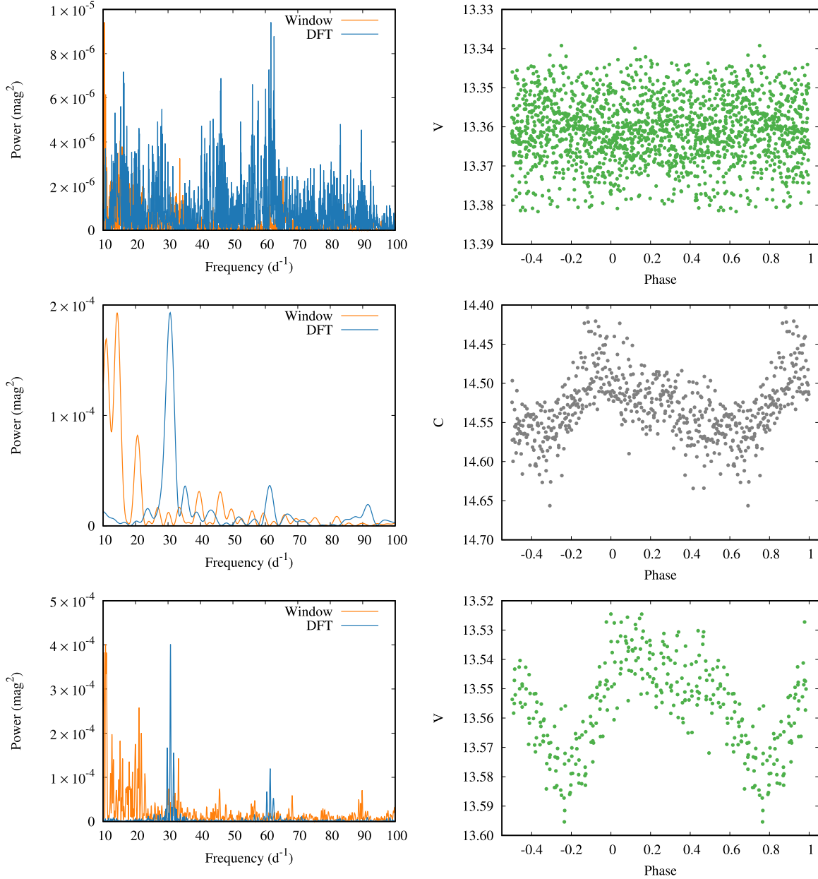
Figure 3. Power spectra with their corresponding spectral windows and phased lightcurves of J0722 during the main outburst (top panels; INASAN-Terskol; V filter), the rise to the rebrightening (middle panels; VSNET Hiroshi Itoh; Clear band) and during rebrightening (bottom panels). All lightcurves are phased with the light elements HJD(TT) = 2460718.3052 + 0.032516 \times E corresponding to the highest peak in the rebrightening power spectrum (bottom left panel; INASAN-Kislovodsk; V filter).
