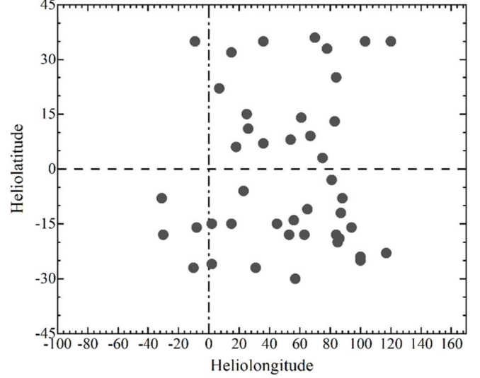
Figure 3. The distribution of GLE event source regions during 1980–2024.
