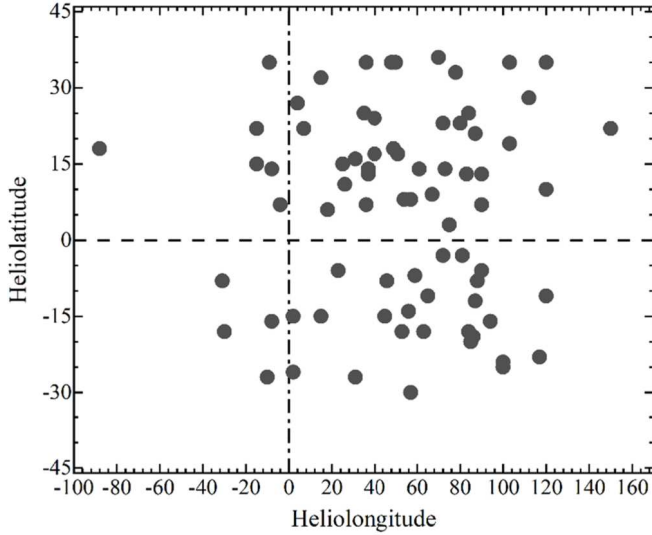
Figure 4. The distribution of GLE event source regions during 1942–2024.
