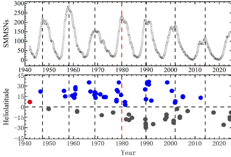
Figure 1. Solar cycle distribution of GLE event heliolatitudes from 1942 to 2024. Blue and black solid circles denote the source locations of GLE events in the Northern and Southern Hemispheres, respectively. For the two GLE events in 1942, we use a blue solid circle to represent the event that occurred on February 8, and a red solid circle to represent the event that occurred on March 7.
