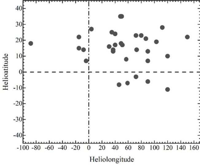
Figure 2. The distribution of GLE event source regions during 1942–1979.
