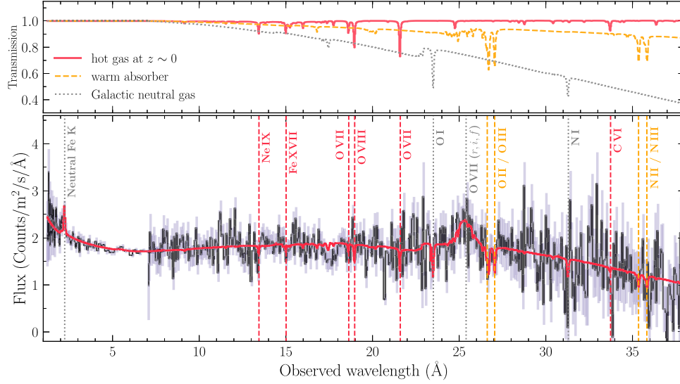
Figure 2. Best-fit spectra using plasma models. The top panel shows the model decomposition of the absorption components. The red solid, orange dashed, and gray dotted lines represent the contributions from the galactic hot halos at z \sim 0 , the WA intrinsic to the AGN, and the Galactic neutral gas absorption, respectively. The black curve and purple bars in the bottom panel are the observed data and the corresponding 1\sigma errors. The best-fit model is shown as the red curve. For clarity, we additionally rebinned the data and displayed only the EPIC-pn and first-order RGS spectra. The prominent line features are labeled by the vertical lines, with the WA and galactic hot-halo lines highlighted in orange and red, respectively.
