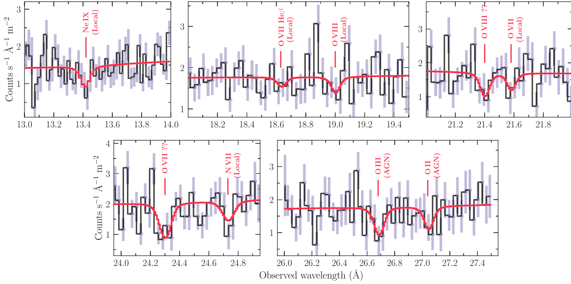
Figure 1. Best-fit segmental spectra of PG 0052+251 by Gaussian line analysis. The black curve is the observed data, with the 1\sigma uncertainty shown in the purple bars. The red curve is the best-fit model. The data are additionally rebinned for display purposes. The absorption features near 13.1 and 21.8 Å are instrumental features of RGS.
