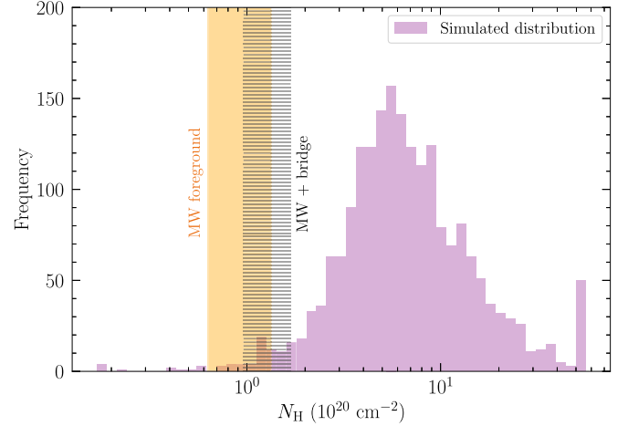
Figure A1. Simulated distribution of the LOS total N_{\text{H}} at zero redshift. The purple histogram represents the N_{\text{H}} distribution obtained by fitting 2000 simulated spectra. This distribution reflects the stochastic scatter of the N_{\text{H}} measurement through the plasma fitting. The orange shaded area indicates the foreground N_{\text{H}} value of the MW, while the gray shadow accounts for contributions from both the MW and the bridge. The total N_{\text{H}} distribution exceeds the MW foreground by 2.2–2.6 \sigma and the combined “MW+bridge” foreground by 2.0–2.4 \sigma , respectively.
