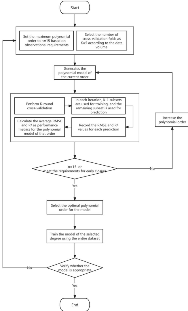
Figure 2. The process of making a polynomial regression model.
