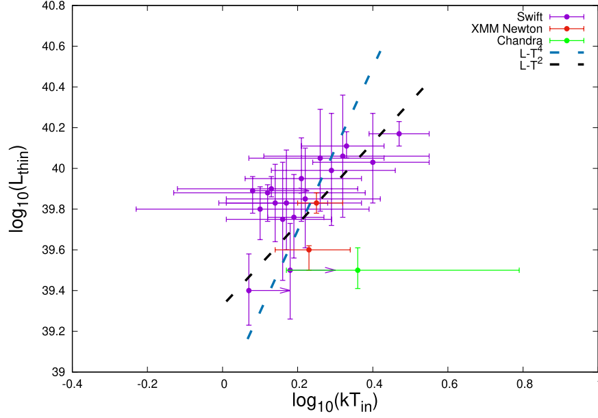
Figure 3. L-T relation for the standard thin disk model.
