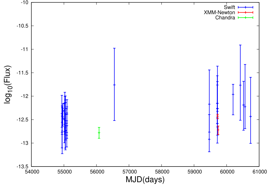
Figure 5. Long term 0.3–10.0 keV flux variation of ULX-1.
