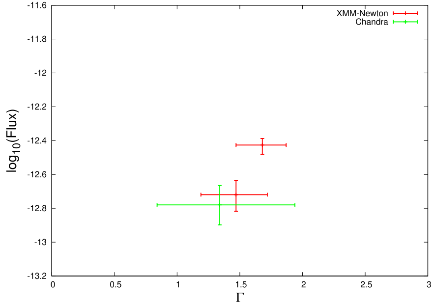
Figure 6. 0.3–10.0 keV flux and spectral hardness relation for XMM-Newton and Chandra data.
