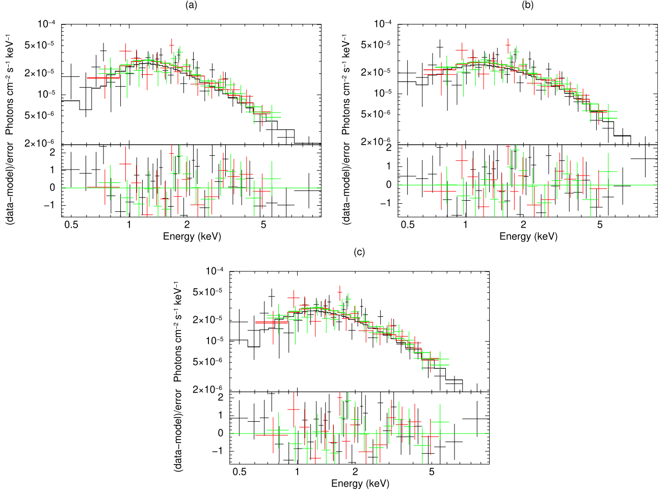
Figure 2. Unfolded spectrum of ULX-1 for the XMM-Newton observation (Obs Id-0882480301) simultaneously fitted with- (a) powerlaw model (b) disk blackbody model and (c) diskpbb model. Black color represents PN data, red color represents MOS1 data and green color represents MOS2 data.
