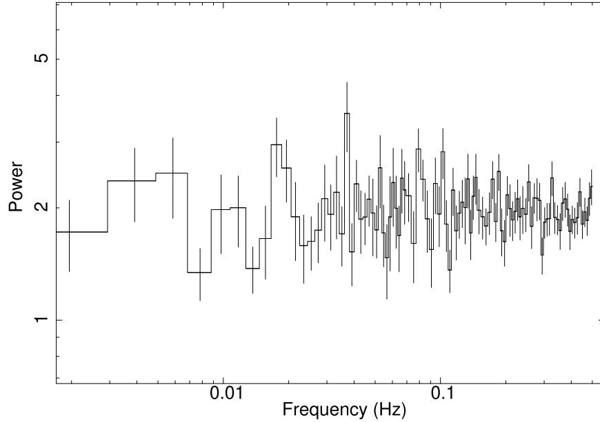
Figure 1. PDS of the source, created using the Leahy normalization for the observation, Obs Id-0882480301, indicating no evidence of any intrinsic variability above the white noise.
