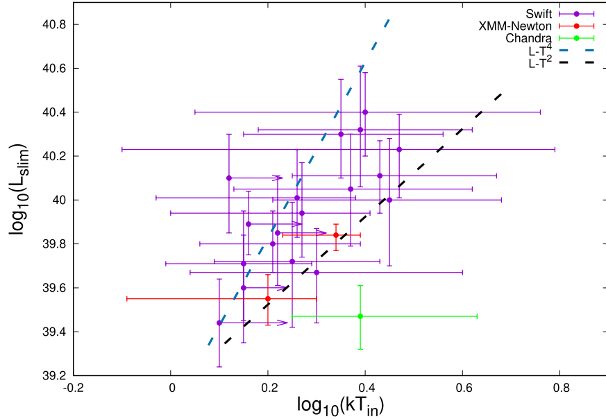
Figure 4. L-T relation for the slim disk model.
