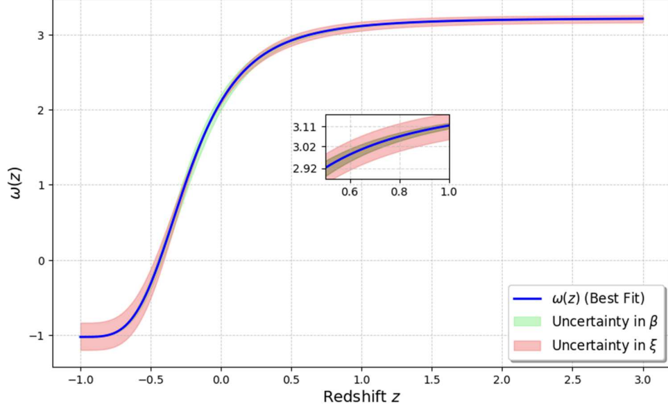
Figure 7. The plot of the EoS parameter \omega(z) vs. redshift z .
