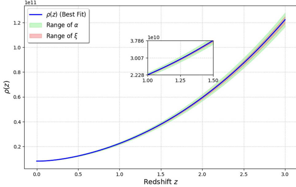
Figure 5. The plot of density \rho(z) vs. redshift z .
