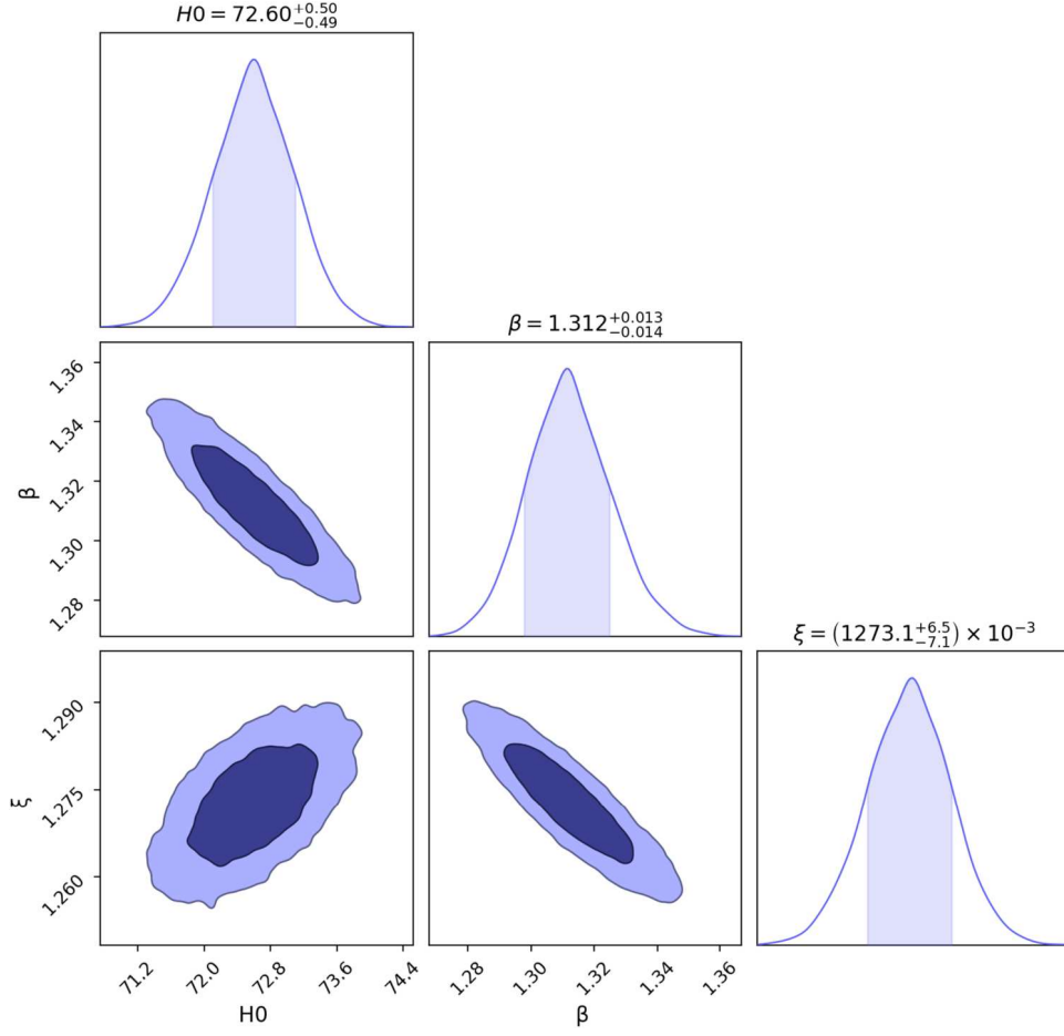
Figure 3. The plot of 1\sigma and 2\sigma confidence intervals using the Hubble, \Lambda CDM, DA, and BAO methods.
