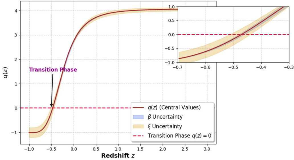
Figure 4. The plot of the deceleration parameter q(z) vs. redshift z .
