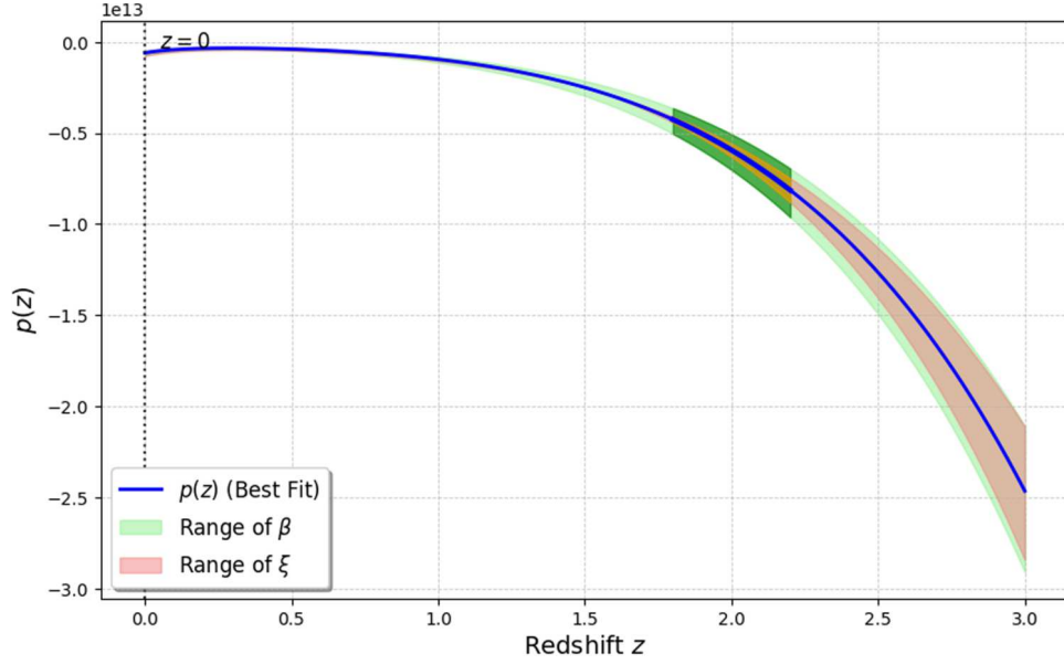
Figure 9. The plot of pressure p(z) vs. redshift z .
