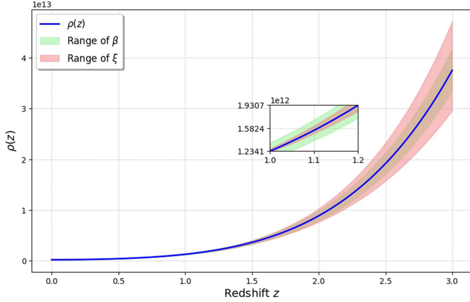
Figure 8. The plot of density \rho(z) vs. redshift z .
