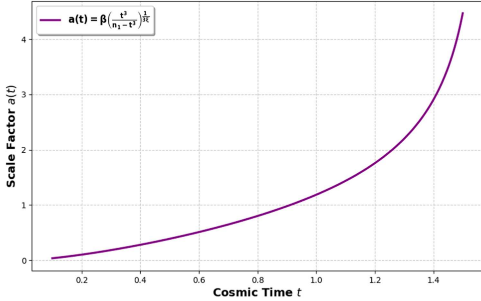
Figure 1. The plot of the scale factor a(t) vs. cosmic time t .
