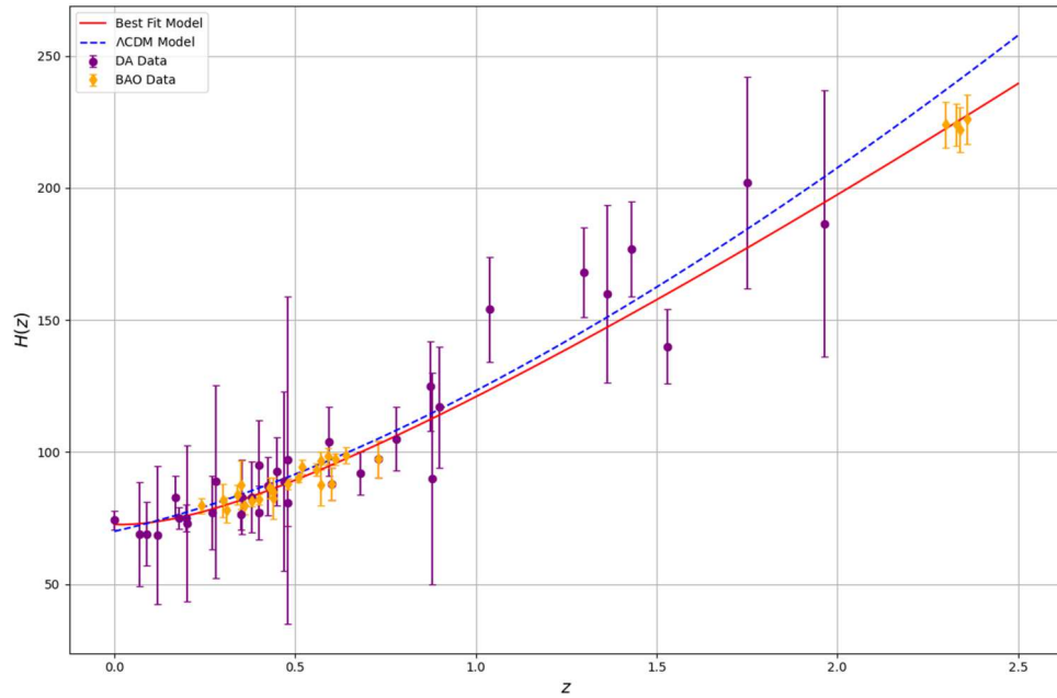
Figure 2. The plot of the Hubble parameter H(z) vs. redshift z , with observational data from the Hubble dataset.
