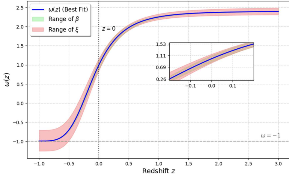
Figure 10. The plot of the EoS parameter \omega(z) vs. redshift z .
