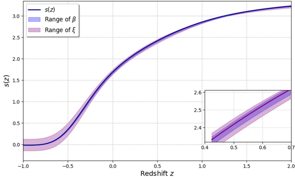
Figure 12. The plot of s(z) vs. redshift z .
