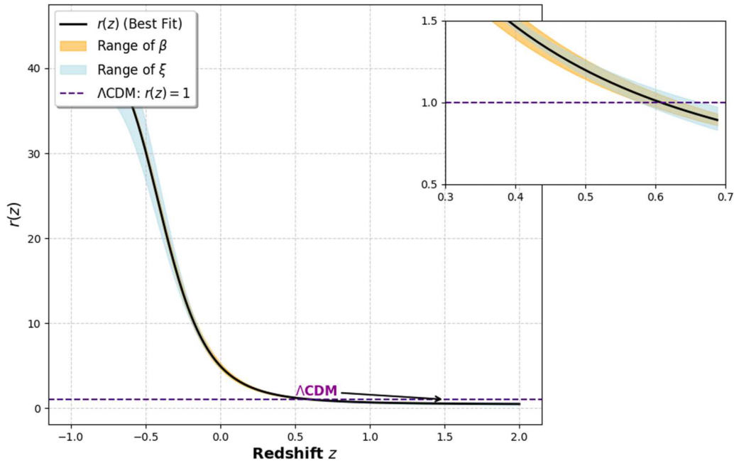
Figure 11. The plot of r(z) vs. redshift z .
