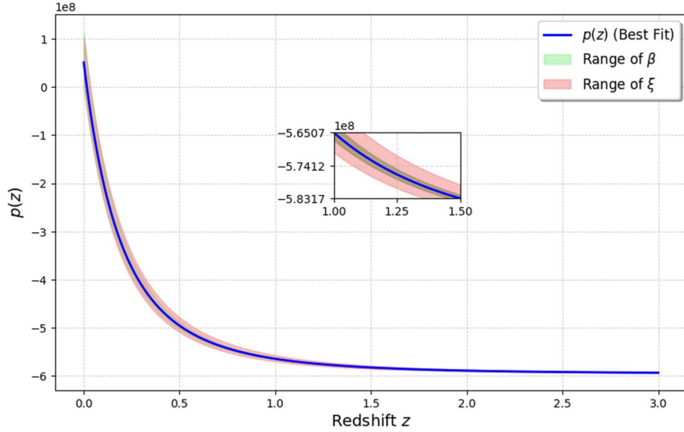
Figure 6. The plot of pressure p(z) vs. redshift z .
