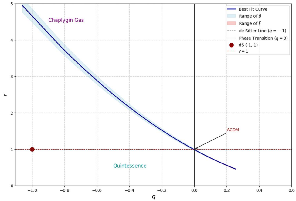
Figure 14. The plot of r(z) vs. q(z) .
