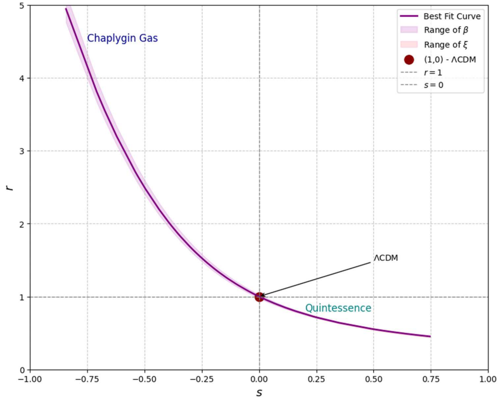
Figure 13. The plot of r(z) vs. s(z) .
