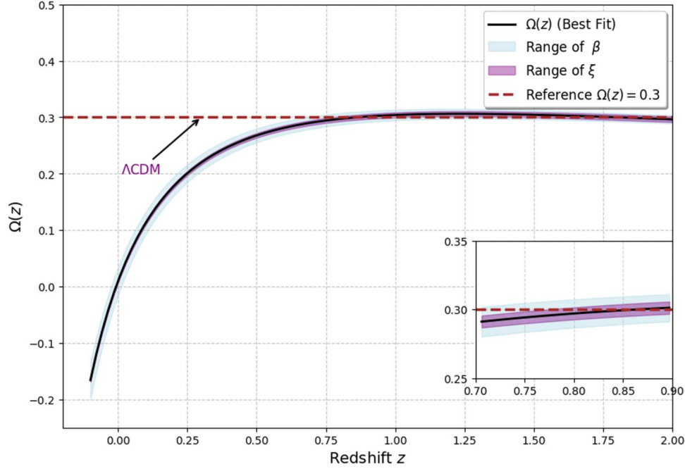
Figure 15. Variation of the Om parameter \Omega(z) with redshift z .
