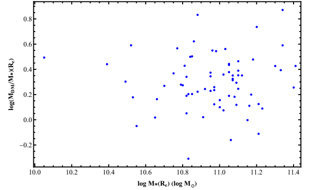
Figure 6. The correlation between M_{\text{DM}} and M_* derived from the sample SLACS.
