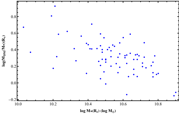
Figure 4. The correlation between M_{\text{DM}} and M_* derived from the sample of SDSS DR 10 (Saulder et al. 2015).
