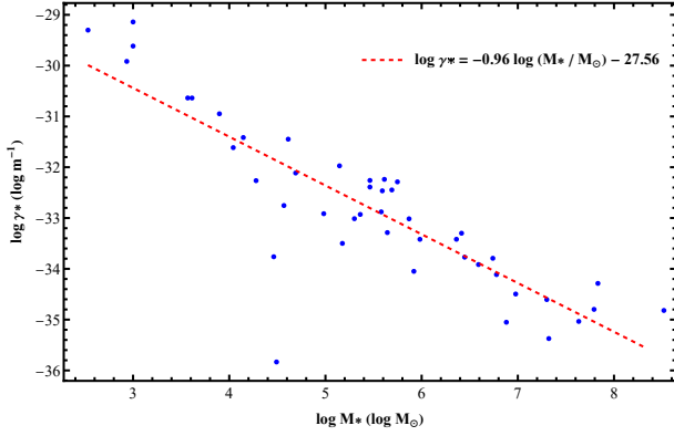
Figure 1. The correlation between the stellar mass M_* and \gamma_{\text{dSph}}^* . The results are obtained based on our selected sample for dSphs. We have set \gamma_0 to 3.97 \times 10^{-29} m^{-1} and calculate \gamma^* at r = R_e using the Jeans Equation (39).
