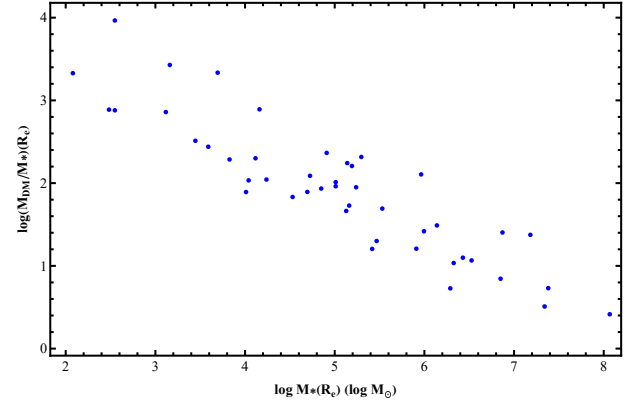
Figure 2. The correlation between M_{\text{DM}} and M_* for the sample of dSphs.
