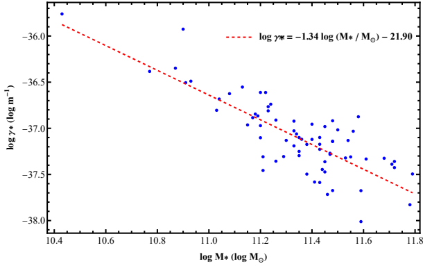
Figure 5. The correlation between \gamma^*_{\text{SLACS}}(R_e) and M_*(R_e) based on the sample SLACS.
