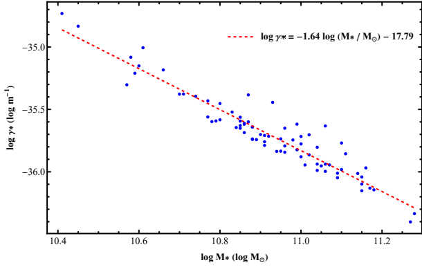
Figure 3. The correlation between \gamma_{\text{SDSS}}^* and M_* based on the sample of SDSS DR 10 (Saulder et al. 2015).
