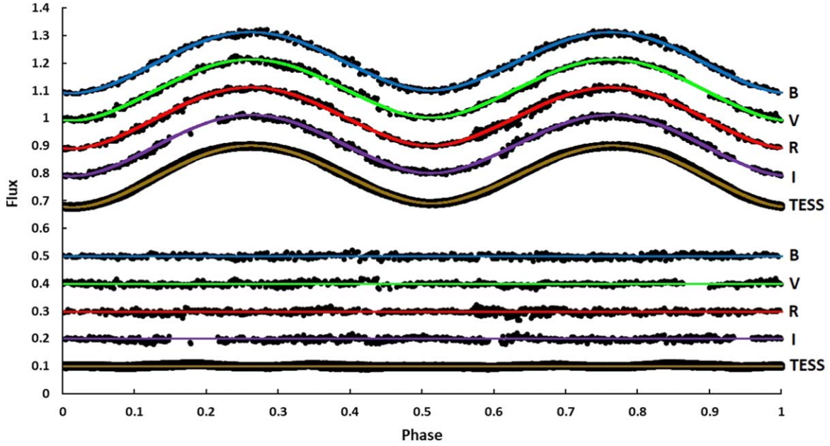
Figure 2. The observed light curves of AP Dor (black dots), and synthetic light curves obtained from light curve solutions in the BVRI filters and TESS (top to bottom respectively), with respect to orbital phase, shifted arbitrarily in the relative flux.
