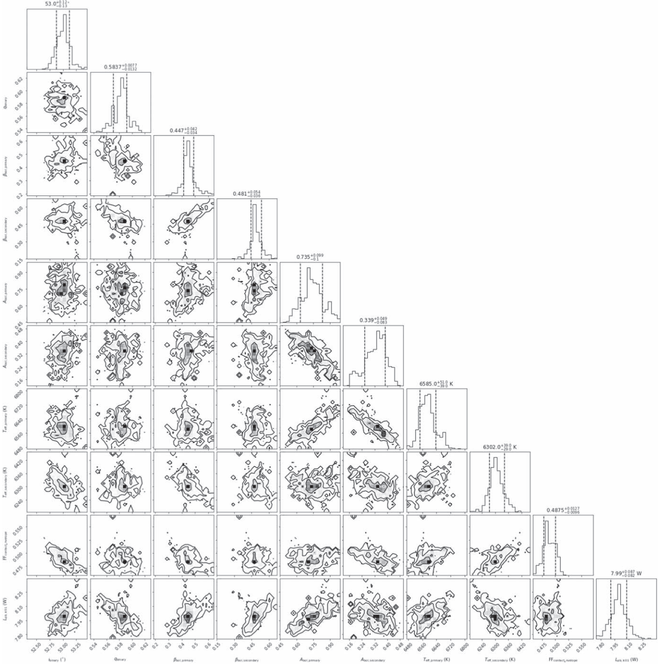
Figure 3. The corner plots of the AP Dor system were determined by MCMC modeling.
