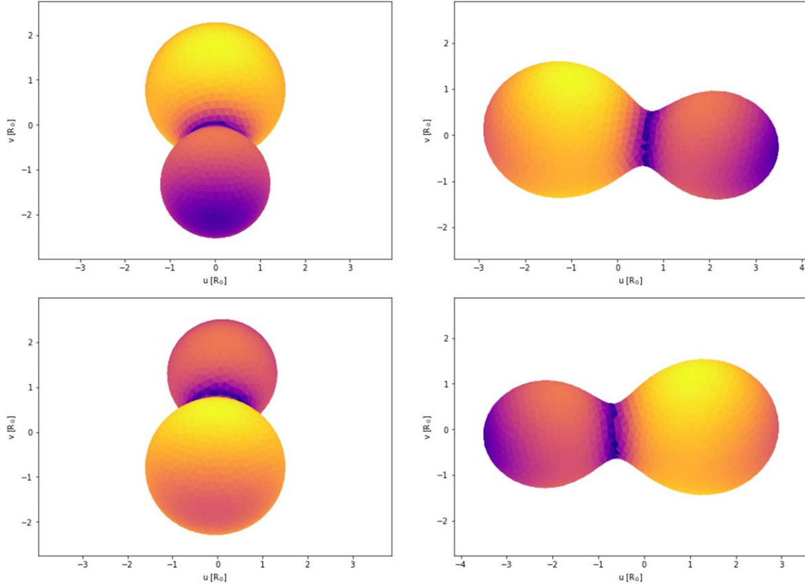
Figure 4. 3D view of stars in the AP Dor system.
