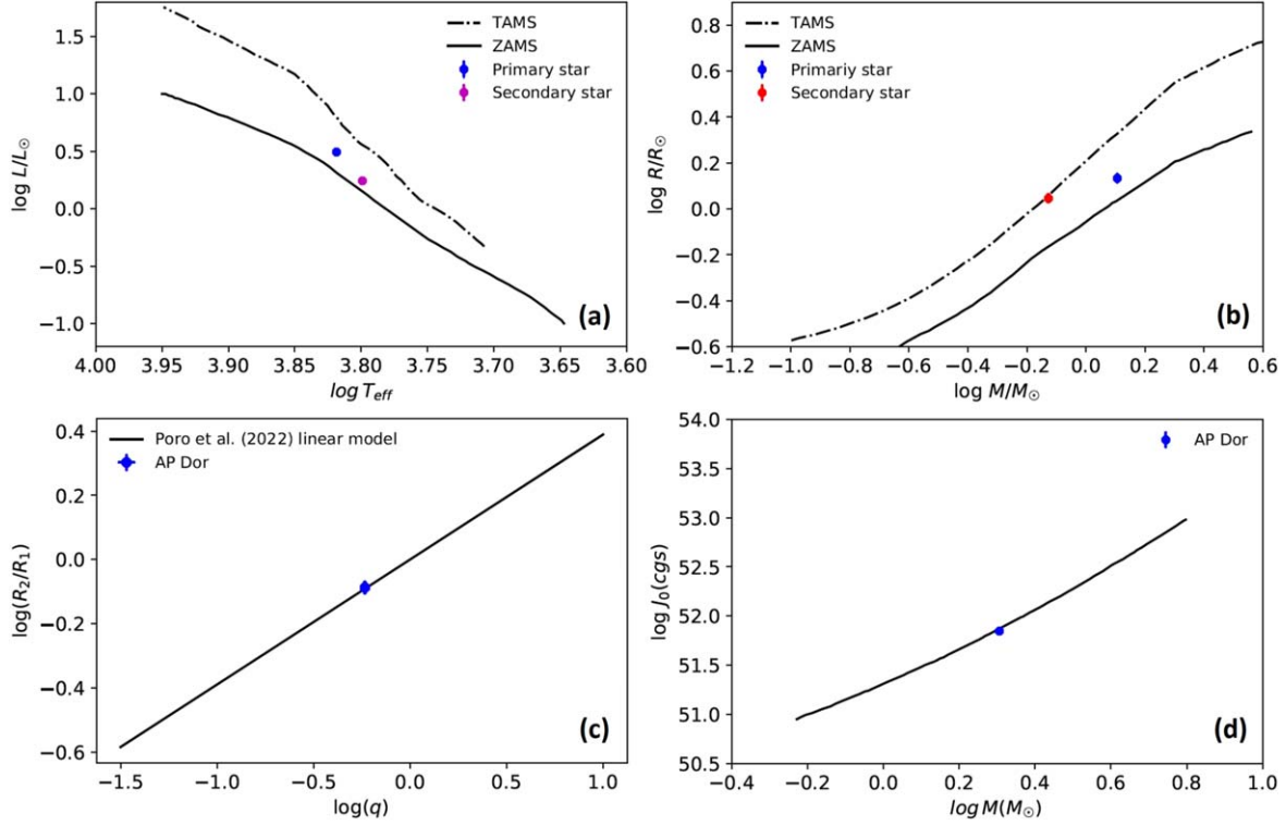
Figure 5. The position of AP Dor on the (a) HR, (b) \log R - \log M , (c) \log R_{\text{ratio}} - \log q , and (d) \log J_0 - \log M diagrams.
