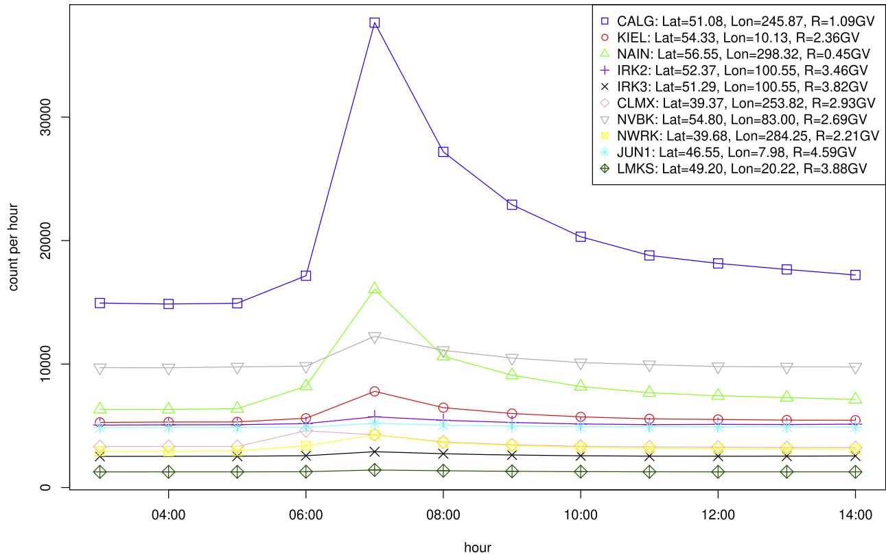
Figure 12. Graph of the GLE 69 hourly CR count at mid-latitudes in the Northern hemisphere.
