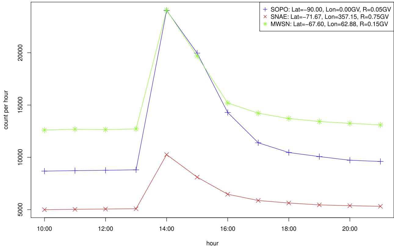
Figure 10. Graph of the GLE 60 hourly CR count at high latitudes in the Southern hemisphere.
