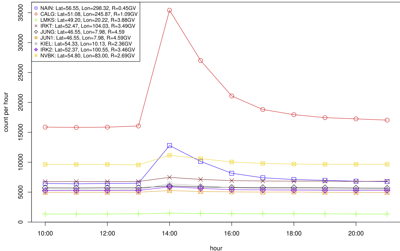
Figure 8. Graph of the GLE 60 hourly CR count at mid-latitudes in the Northern hemisphere.
