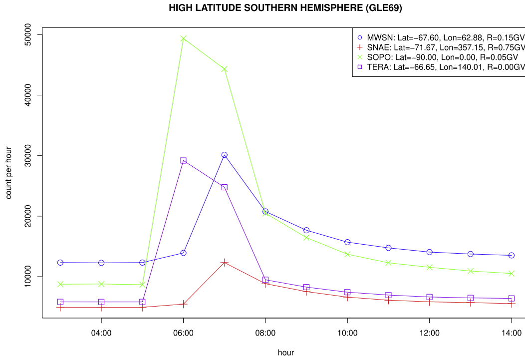
Figure 14. Graph of the GLE 69 hourly CR count at high latitudes in the Southern hemisphere.
