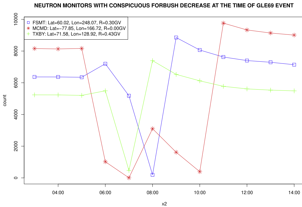
Figure 15. Graph of Concurrent FD with GLE 69.
