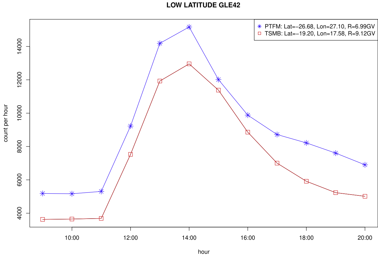
Figure 6. Graph of the GLE 42 hourly CR count at low latitudes.
