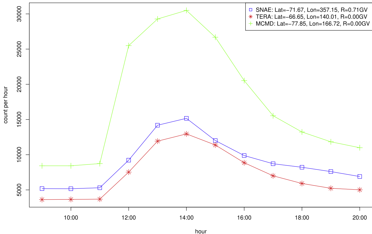
Figure 5. Graph of the GLE 42 hourly CR count at high latitudes in the Southern hemisphere.
