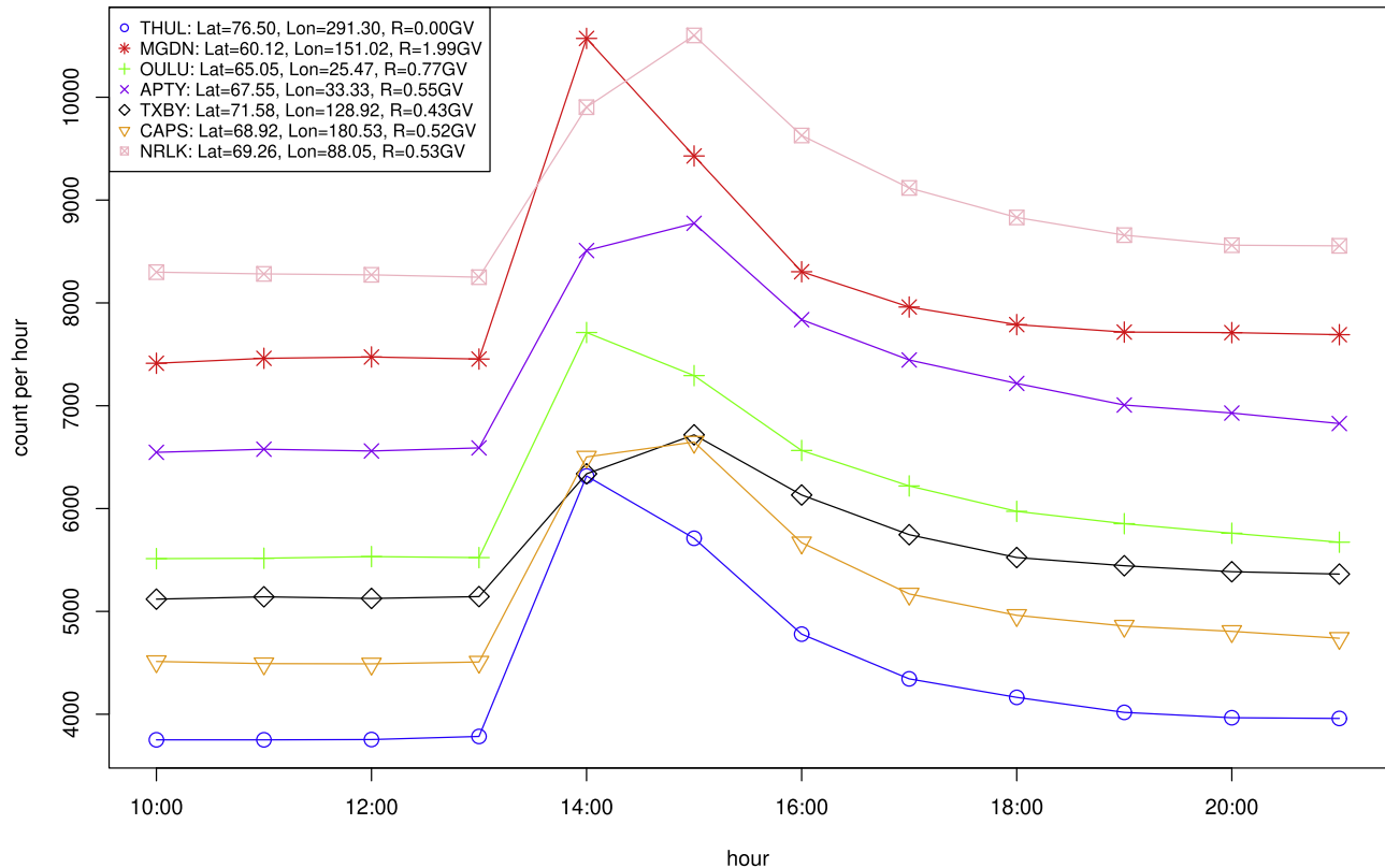
Figure 7. Graph of the GLE 60 hourly CR count at high latitudes in the Northern hemisphere.
