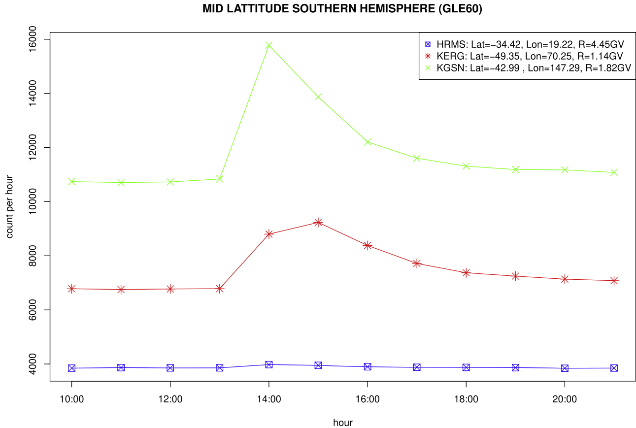
Figure 9. Graph of the GLE 60 hourly CR count at mid-latitudes in the Southern hemisphere.
