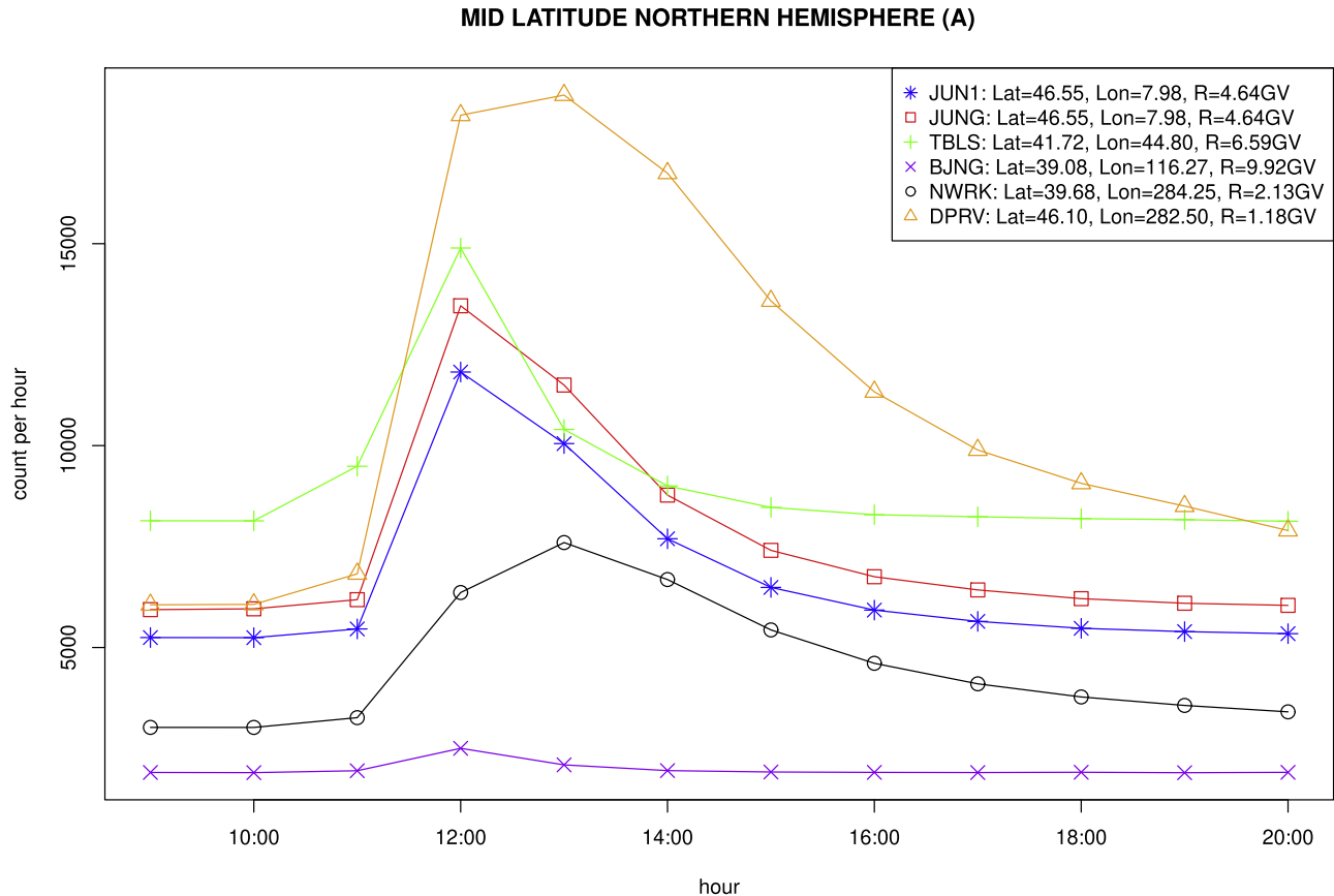
Figure 3. Graph of the GLE 42 hourly CR count at lower mid-latitudes in the Northern hemisphere.
