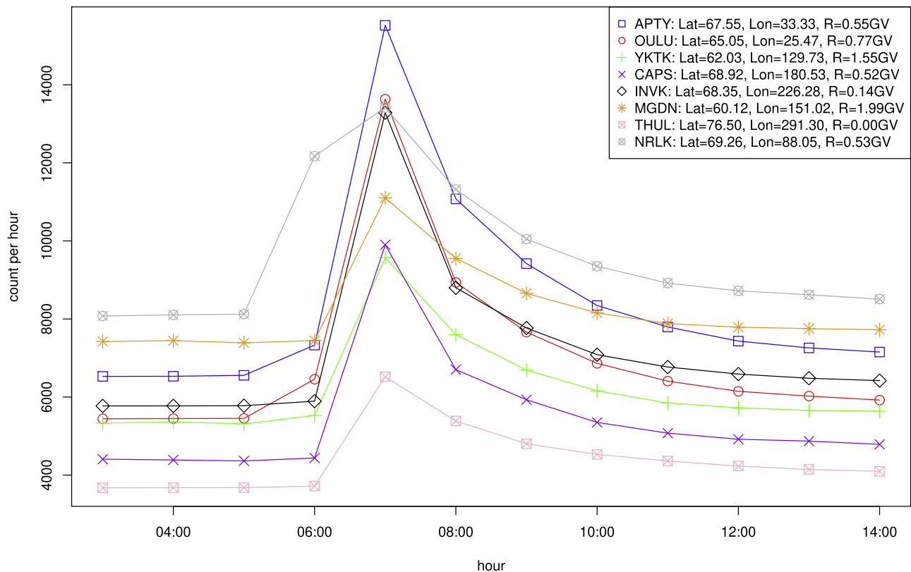
Figure 11. Graph of the GLE 69 hourly CR count at high latitudes in the Northern hemisphere.
