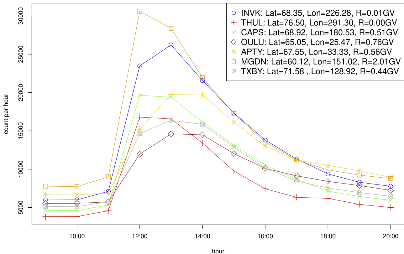
Figure 1. Graph of the GLE 42 hourly CR count at high latitudes in the Northern hemisphere.
