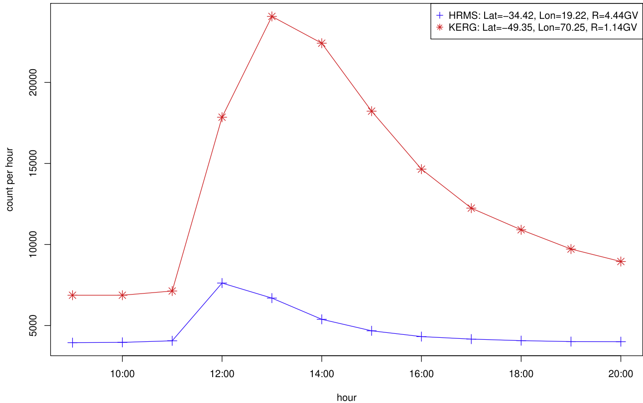
Figure 4. Graph of the GLE 42 hourly CR count at mid-latitudes in the Southern hemisphere.
