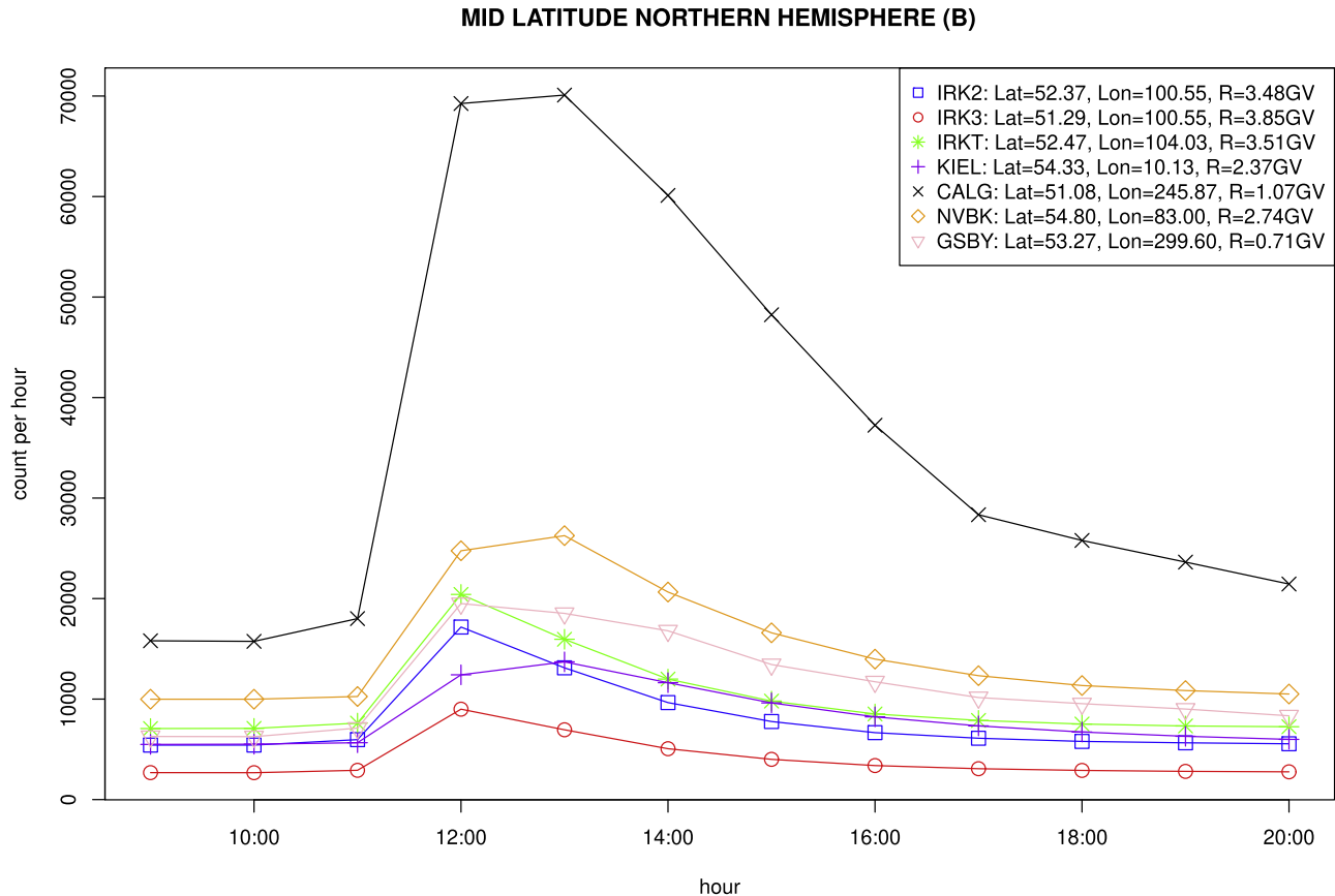
Figure 2. Graph of the GLE 42 hourly CR count at upper mid-latitudes in the Northern hemisphere.
