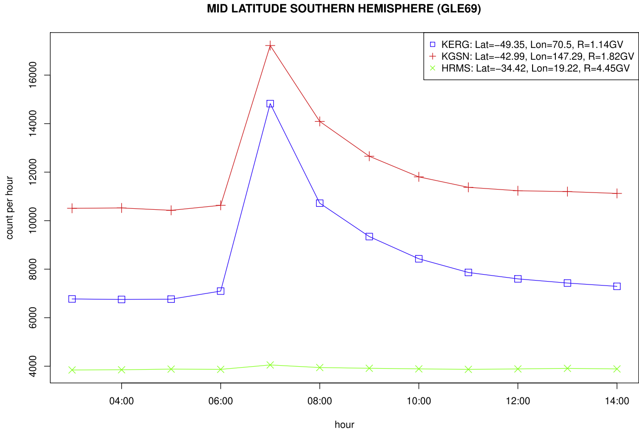
Figure 13. Graph of the GLE 69 hourly CR count at mid-latitudes in the Southern hemisphere.
