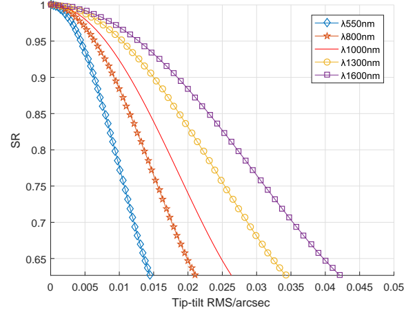
Fig. 6 Relation between SR and the RMS value of tip-tilt at different wavelengths.
