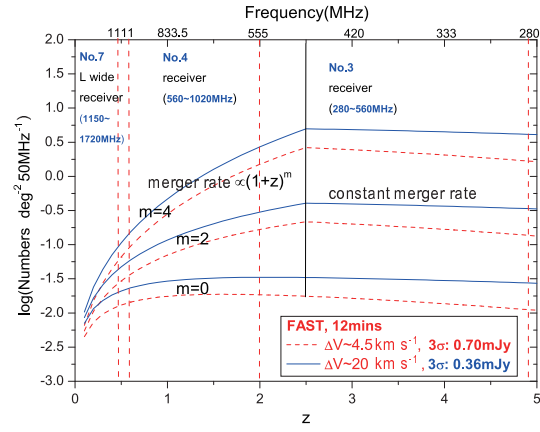
Fig. 2 Detection rate of OH megamasers as a function of redshift (or frequency) with FAST 12 min integration ( dashed lines : 3\sigma \sim 0.7 \text{ mJy} and solid lines : 3\sigma \sim 0.36 \text{ mJy} ): m = 0 for constant merger rate; m = 2 and 4 for merger rate proportional to (1+z)^2 and (1+z)^4 respectively. The solid vertical line indicates the turnover redshift for merger rate ( z = 2.5 ). The frequency ranges of three FAST receivers are also indicated in dashed lines .
