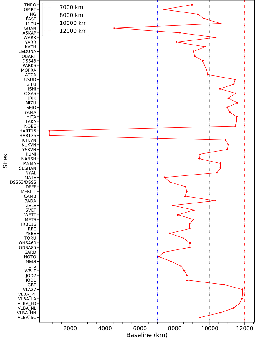
Fig. 5: Distribution of the baseline lengths of all sites against SKA-Mid. The blue, green, black and red vertical lines show baselines of 7000, 8000, 10,000 and 12,000 km, respectively.
