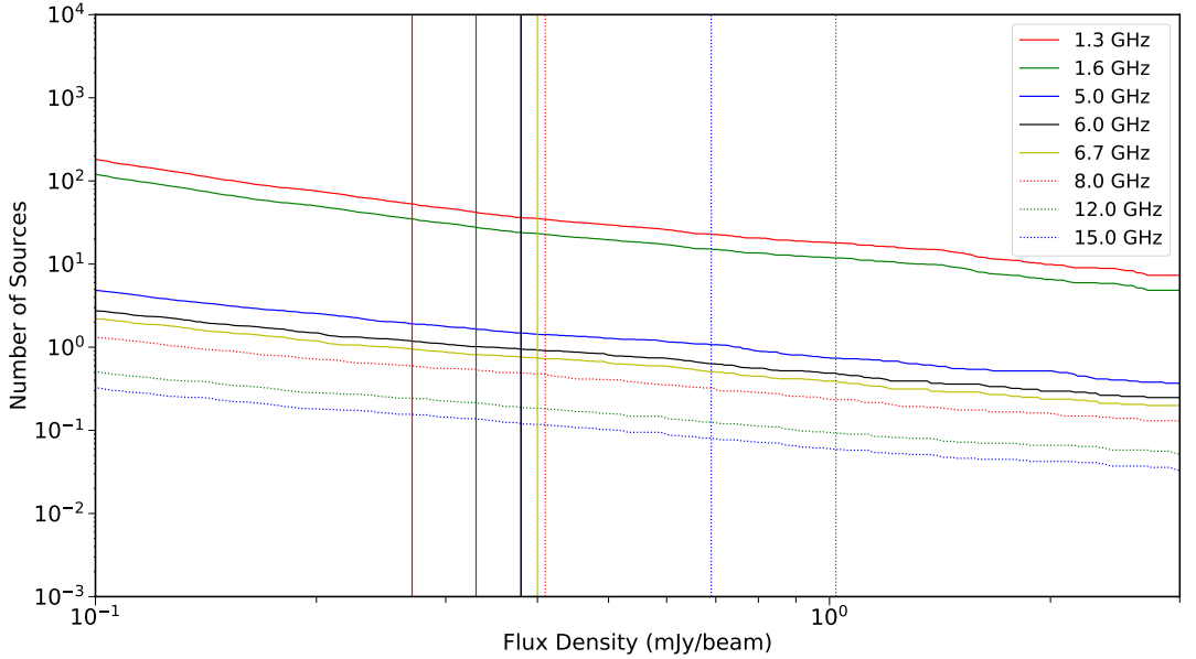
Fig. 6: Number of in-beam sources. The vertical lines shows the sensitivity matched DR of 100:1 (see \Delta S values listed in Table 3), where the lines for 5 and 6 GHz are overlap.
