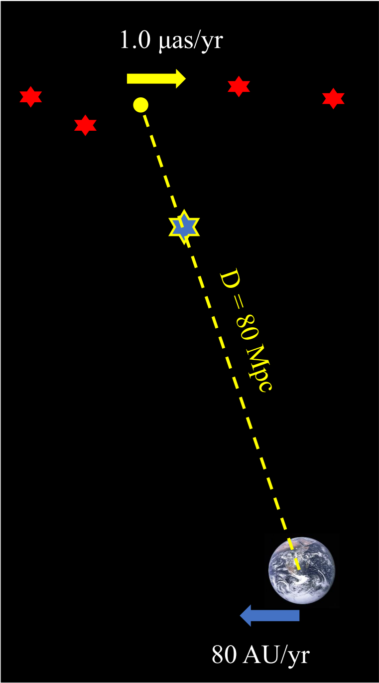
Fig. 11: Schematic showing how geometrical distances can be obtained using Earth’s motion with respect to the CMB as a baseline. In this model, no motion of a extragalactic object with respect to the CMB and the motion of the Earth of 80 \text{ AU yr}^{-1} with respect to the center of the CMB is assumed. With a theoretical proper motion precision of 0.2 \mu\text{as yr}^{-1} achievable through 10 yr of monitoring observations, the distance to an external galaxy 80 Mpc away could be determined with a \sim 20\% error (corresponding to a proper motion of 1.0 \mu\text{as yr}^{-1} ). The icon of Earth is from NASA/Apollo 17 crew, see https://www.nasa.gov/image-article/earth-full-view-from-apollo-17/ .
