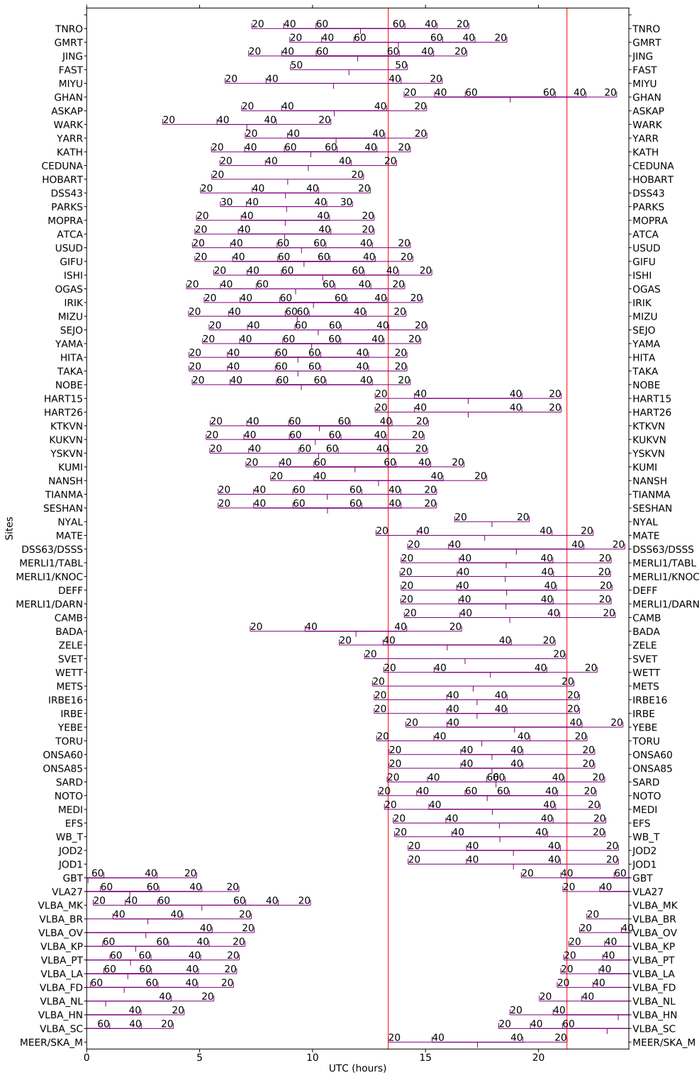
Fig. 3: The distribution of elevation for target sources with Decl. (J2000) of 10^\circ . The red vertical lines indicate the UTC time range with the elevation of SKA-Mid (which is labeled as “SKA_M”) being 20^\circ .
