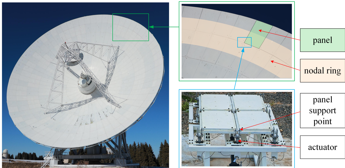
Figure 3. Panel nodes and actuators for reflector antenna.
