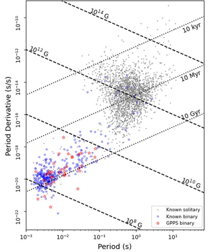
Figure 11. Binary pulsars in the period vs. period derivative diagram. Gray dots represent solidly single pulsars listed in the ATNF pulsar catalog (Manchester et al. 2005). Binary pulsars are indicated by circles. The newly discovered 38 binary pulsars by the GPPS survey which have timing solutions already are indicated by red stars. Dashed and dotted lines represent constant surface magnetic field and characteristic age, respectively.
