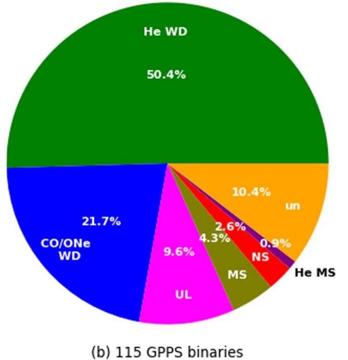
Figure 4. Fractions of binary pulsars with different types of companions in the Galactic field. The top panel is for 315 known binaries and the bottom panel is for the 115 GPPS-discovered ones. Their numbers are listed in Table 6.
