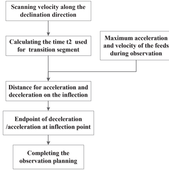
Fig. 9 Motion planning process of the motion scan along the right ascension direction.
