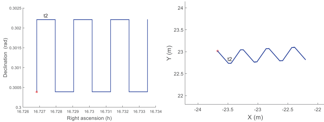
Fig. 8 A sample observation trajectory along the right ascension direction.
