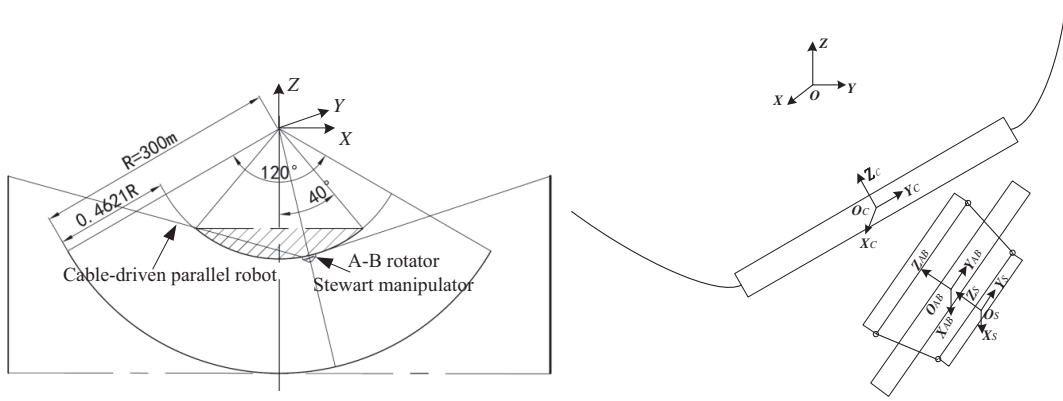
Fig. 3 Main mechanisms of the feed support system.
