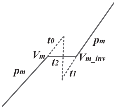
Fig. 13 Related parameters of t_2 in the Cartesian coordinate system.
