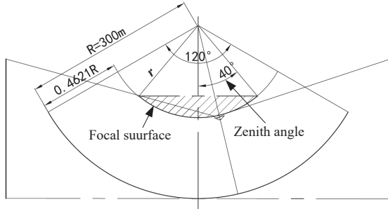
Fig. 14 A sketch map of the feed support system.
