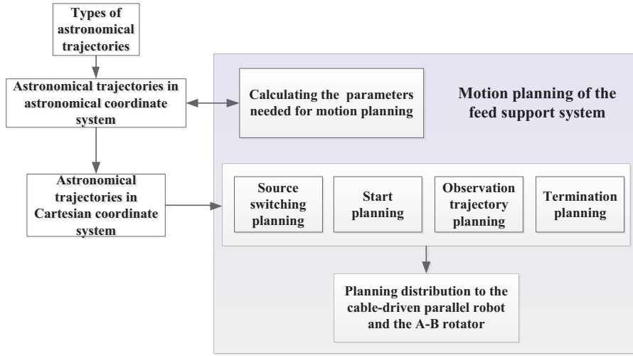
Fig. 4 Motion planning process of the feed support system.
