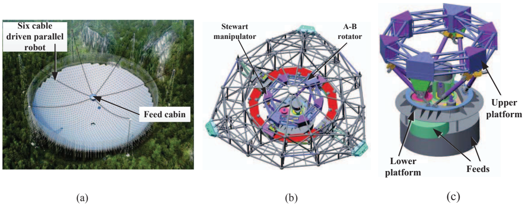
Fig.2 Feed support system. (a) Design of the feed support system for FAST; (b) Feed cabin; (c) Stewart manipulator.
