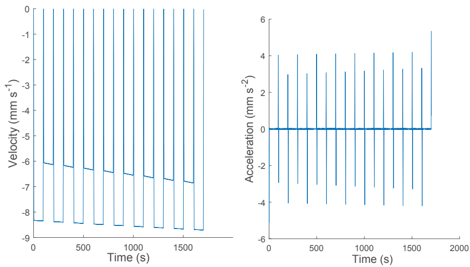
Fig. 17 A motion planning result for the cable driven parallel robot. Left : The velocity of the trajectory; Right : The acceleration of the trajectory.
