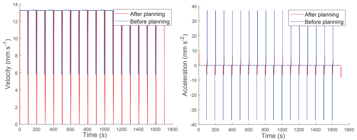
Fig. 16 A motion planning result of a motion scan trajectory along the right ascension direction with start and termination planning. Left : The velocity of the trajectory; Right : The acceleration of the trajectory.
