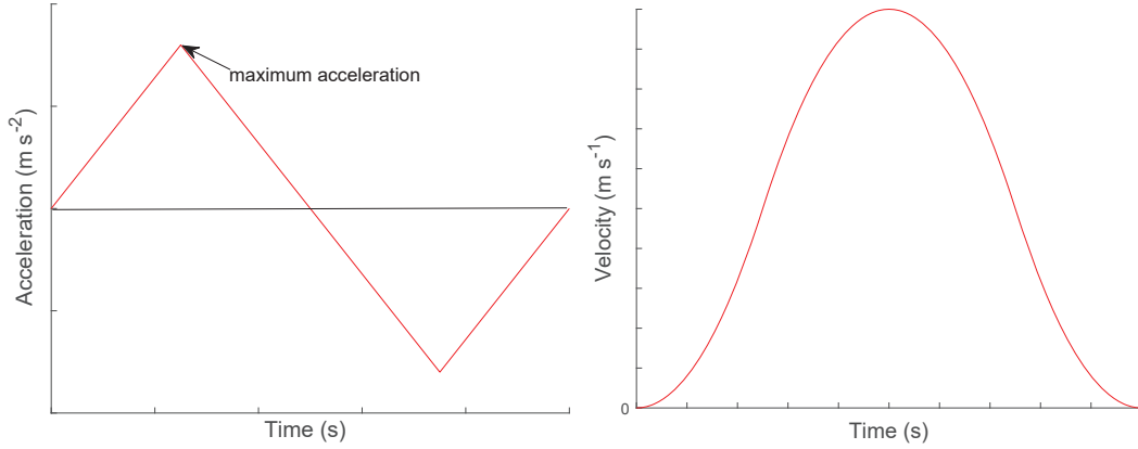
Fig. 6 Acceleration and velocity planning curves.
