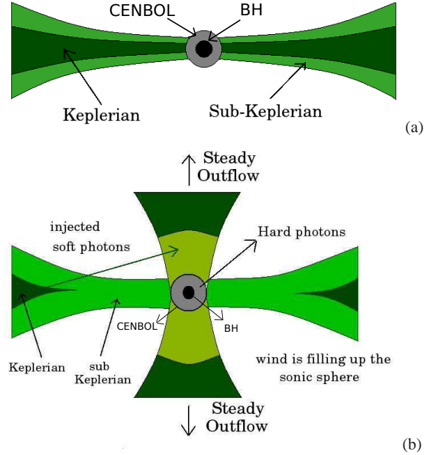
Fig. 1 (a) The accretion flow consisting of Keplerian and sub-Keplerian flow. Their relative abundance dictates the hardness and softness of the state. This configuration corresponds to the \chi_{2,4} classes. (b) A shock is produced due to satisfaction of Rankine-Hugoniot conditions. In both of the figures, the grey shaded region around the BH represents the CENBOL. Outflow is generated and a steady outflow rate is maintained because the average optical depth within the sonic sphere is smaller than unity. This corresponds to the \chi_{1,3} classes (adopted from Chakrabarti et al. 2000).
