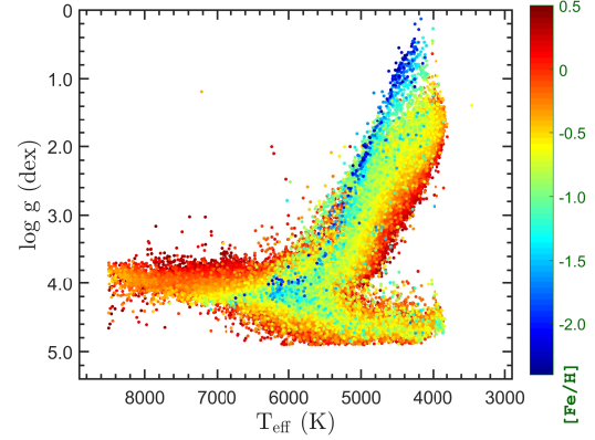
Fig. 5 Kiel diagram ( \log g vs. T_{\text{eff}} ) of the “qualified” LK spectra. The parameters are derived from the LASP pipeline. Note that different colors indicate different values of metallicity [\text{Fe}/\text{H}] .
