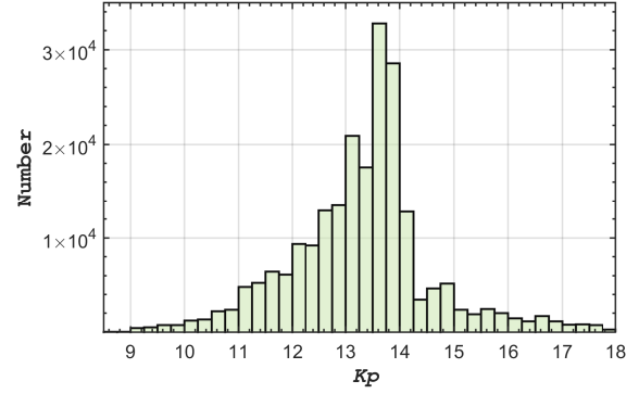
Fig. 2 Distribution of the Kepler magnitude of the stars observed by LAMOST during phase I of the LK project.
