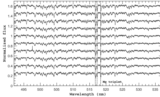
Fig. 9 Examples of LAMOST medium-resolution spectra of the object KIC 08685306 in blue band. These 10 time-domain spectra were obtained in two nights from the LK-MRS survey, with quality of S/N \sim 50 . Flux of these spectra is normalized and shifted with relative values for visualization. The most distinct absorption lines for instance the Magnesium (Mg) triplet are marked with vertical lines.
