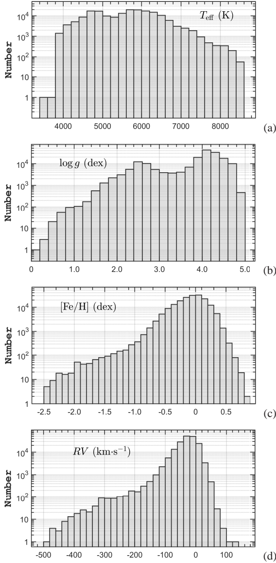
Fig. 4 Histogram of atmospheric parameters and RV derived from 238 386 spectra. Panel (a): the effective temperature T_{\text{eff}} (K); (b): the surface gravity \log g (dex); (c): the metallicity [\text{Fe}/\text{H}] (dex); and (d): the radial velocity RV ( \text{km s}^{-1} ).
