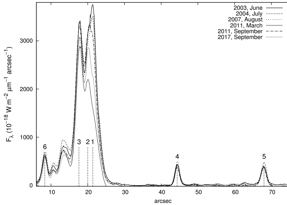
Fig. 3 Superposition of the flux density profiles along the rectangle shown in Fig. 1. The designations are similar to those in Fig. 1 and Fig. 2. Star 4 was used for calibration and stars 5 and 6 for calibration control. All data are smoothed to the angular resolution of CMO. Source 1 was significantly fainter in March 2011 and September 2017 with respect to the other epochs.
