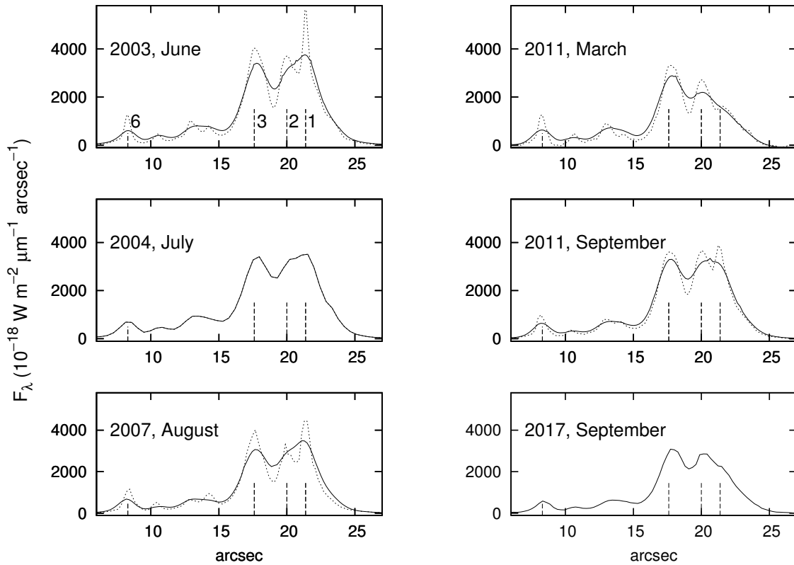
Fig. 2 The flux density distribution along the rectangle shown in Fig. 1. The vertical scale is rough and was obtained from the K = 14.525 mag 2MASS catalog value for star 4. The horizontal scale represents the angular distance (in arcsecond) from (J2000): RA = 18^{\text{h}}34^{\text{m}}20.952^{\text{s}} and Dec = -5^{\circ}59'25.375'' . The solid line represents data after smoothing to the CMO angular resolution, and dotted line corresponds to data without angular smoothing (for cases when the angular resolution of the data is different from the CMO data one). The dashed bar marked by 1 indicates peak position of the IR source nearest to the water maser. The positions of sources, marked by dashed bars in all panels, are taken from the peak positions of the first panel image (2003–06–16, data with better angular resolution). The source designations are the same as in Fig. 1. The K -band intensity of source 1 was significantly less in March 2011 and September 2017 with respect to other epochs.
