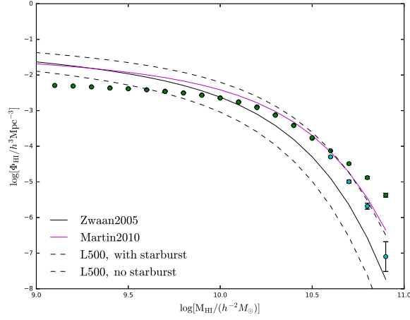
Fig. 11 The HI mass functions: green dots are our fiducial model predictions, while cyan dots are the model predictions that take into account the starburst. The black solid line shows the best fit observational results obtained by Zwaan et al. (2005) with dashed lines that indicate the associated \pm 1\sigma scatter. The magenta curve is the observational fitting formula obtained by Martin et al. (2010).
