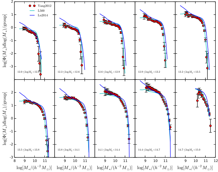
Fig. 5 Similar to Fig. 3 but for satellite galaxies.
