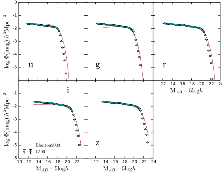
Fig. 7 LFs of galaxies in the u, g, r, i, z band at z = 0.1 . The solid curve in each panel is the corresponding best fit Schechter LF obtained by Blanton et al. (2003) from SDSS DR1.
