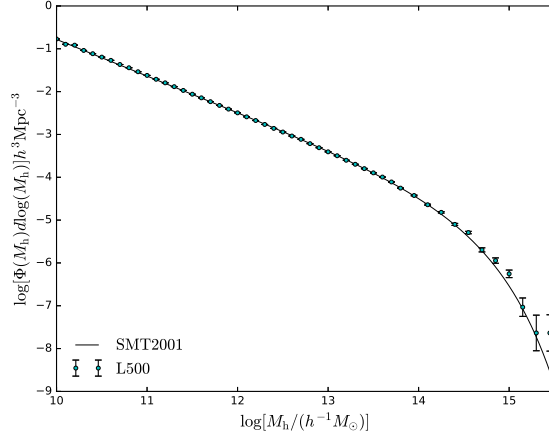
Fig. 1 Halo mass functions of the simulation. The black curve and cyan circles represent respectively the SMT2001 analytic prediction and data extracted from the L500 simulation.
