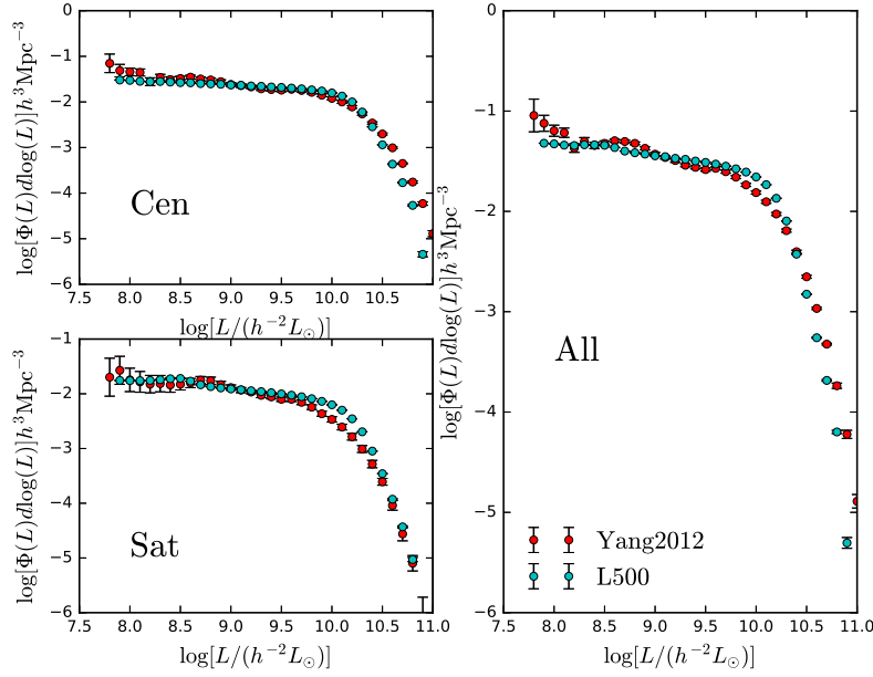
Fig. 8 LFs of central, satellite and all galaxies in the r band in the local universe. Here results are shown for observational measurements ( red dots ) and our fiducial model predictions ( cyan dots ).
