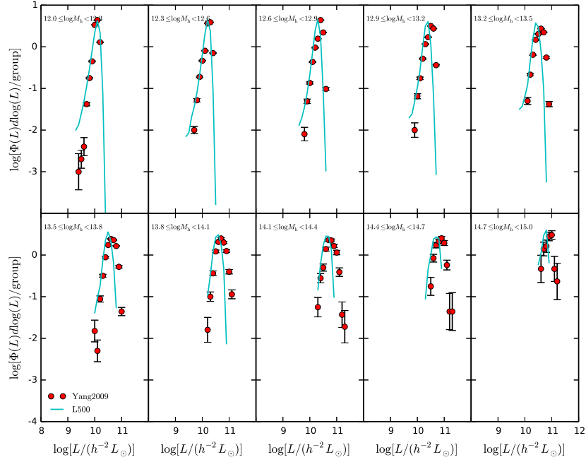
Fig. 9 CLFs of central galaxies in halos with different mass bins. Here results are shown for observational measurements ( red dots ) and our fiducial model predictions ( cyan curves ).
