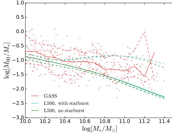
Fig. 12 The HI-to-stellar mass ratios as a function of galaxy stellar mass. Here red points are data from the GASS (Catinella et al. 2013) compilation. Red curves are the median ( solid ) and 68% confidence range ( dashed ) of the ratio in the GASS sample. Green and cyan curves represent the median ( solid ) and 68% confidence range ( dashed ) of our fiducial and starburst model predictions, respectively.
