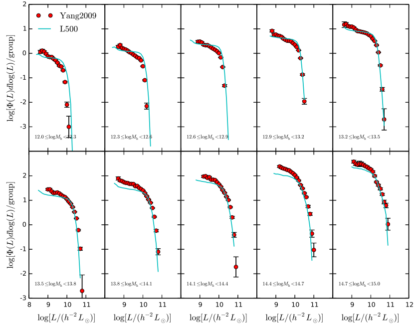
Fig. 10 Similar to Fig. 9 but for the satellite galaxies.
