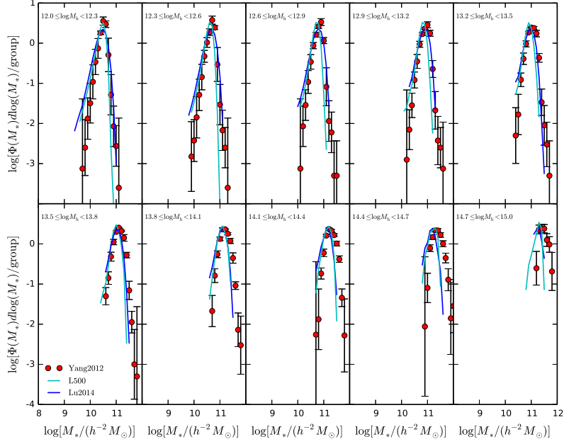
Fig. 4 CSMFs of central galaxies. Different panels correspond to different halo mass bins as indicated. The cyan curves are the CSMFs of our EM, while blue curves are obtained using the Lu14 SFH model. Red filled circles with error bars are the CSMFs of SDSS DR7 obtained by Yang et al. (2012).
