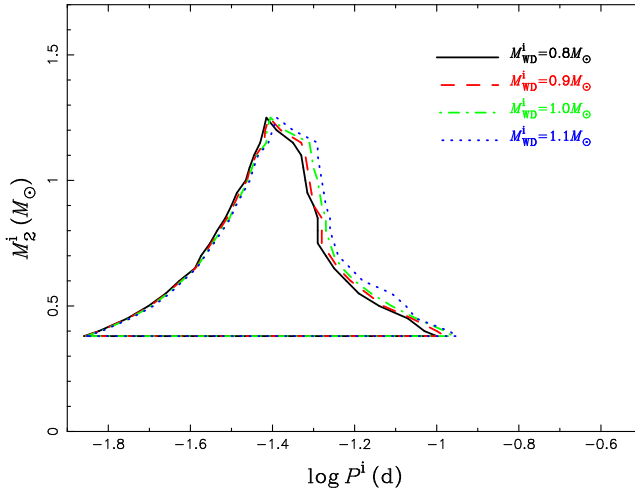
Fig. 2 Space parameters in the initial orbital period–secondary mass plane ( \log P^i, M_2^i ) for CO WD + He star binaries that produce SNe Ia with various initial WD masses.
