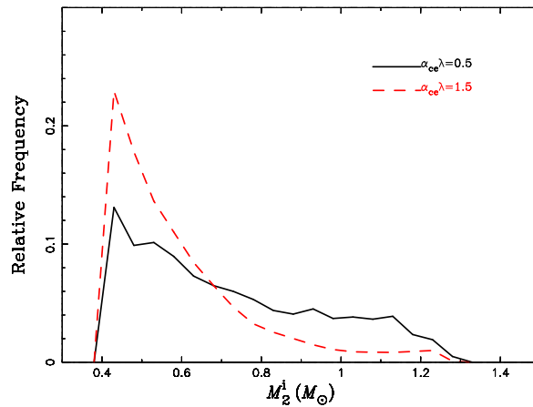
Fig. 6 Similar to Fig. 5, but for the distribution of the initial masses of secondaries in the WD + He star systems.
