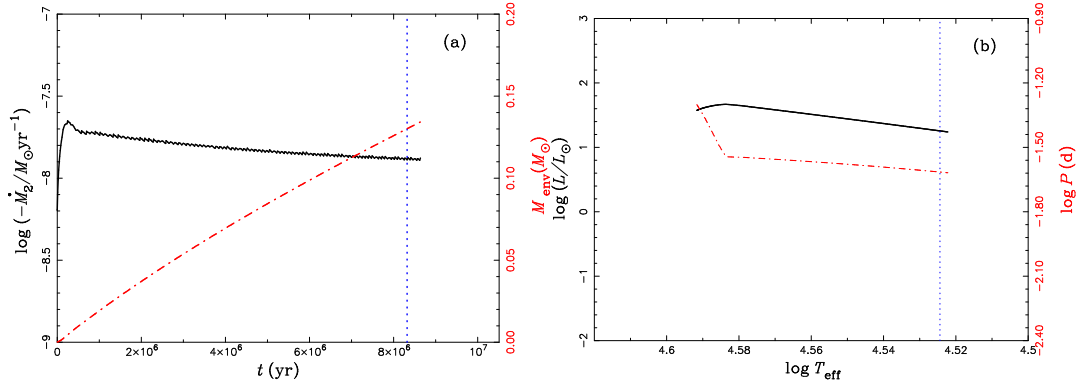
Fig. 1 A typical example of a binary evolution calculation. (a) The solid and dash-dotted curves show the mass-transfer rate and the mass of the He layer on the WD varying with time after the He star fills its Roche lobe, respectively. (b) The evolutionary track of the donor star is shown as a solid curve and the evolution of orbital period is shown as a dash-dotted curve. In this binary, the initial mass of the WD is 0.9 M_\odot , the initial mass of the He star is 0.6 M_\odot , and the initial period is about 0.05 d; the final mass of the He star is 0.47 M_\odot , and the final period is about 0.025 d when the mass of the envelope increases to 0.13 M_\odot .
