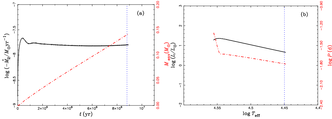
Fig. 8 Similar to Fig. 1, but for the results of binary evolution calculations corresponding to the binary system CD–30 11223. In this binary, the initial mass of the WD is 0.76 M_{\odot} , the initial mass of the He star is 0.51 M_{\odot} , and the initial period is about 0.05 d; the final mass of the He star is 0.37 M_{\odot} , and the final period is about 0.017 d when the mass of the envelope increases to 0.14 M_{\odot} .
