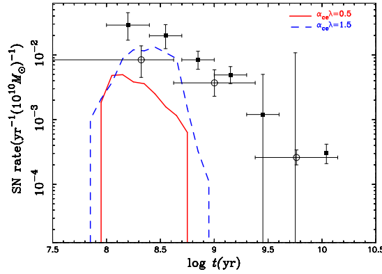
Fig. 4 Delay time distributions of SNe Ia for the double-detonation model. The open circles and filled squares are taken from Maoz et al. (2011) and Totani et al. (2008), respectively.
