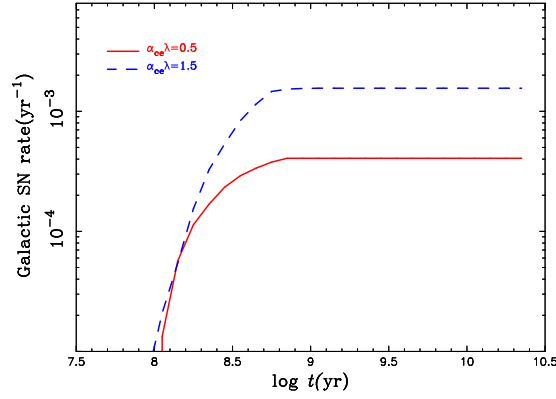
Fig. 3 Evolution of Galactic SN Ia birthrates for a constant star-formation rate.
