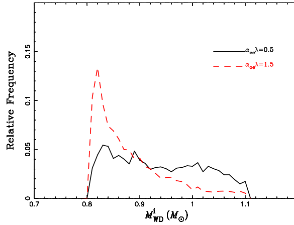
Fig. 5 Distribution of the initial WD masses in the WD + He star systems that can ultimately produce double-detonation explosions.
