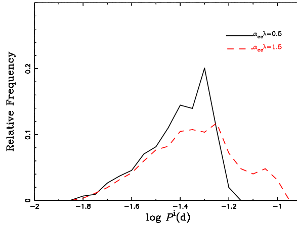
Fig. 7 Similar to Fig. 5, but for the distribution of initial orbital periods of the WD + He star systems.
