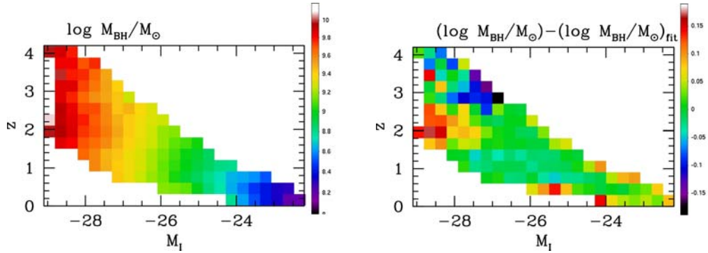
Fig. 1 (Left) Average of \log_{10} M_{\text{BH}} (logarithm of the black hole mass) in bins of \Delta z = 0.3 in redshift and \Delta M_i = 0.3 in the i -rest absolute magnitude. (Right) Difference between the data and the best fit model.
