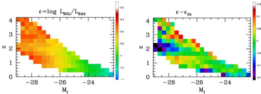
Fig. 2 (Left) Average of \log_{10} \epsilon (logarithm of the Eddington ratio) in bins of \Delta z = 0.3 in redshift and \Delta M_i = 0.3 in the i -rest absolute magnitude. (Right) Difference between the data and the best fit model.
