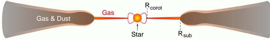
Fig. 1 Illustration of the structure in the inner regions of the circumstellar disk around a solar-mass young stellar object in the classical T Tauri stage. Typical sizes are: R_* \sim 2 R_\odot , R_{\text{corot}} \sim 3-10 R_* , R_{\text{sub}} \sim 0.1 \text{ AU} (\sim 10 R_*) .
