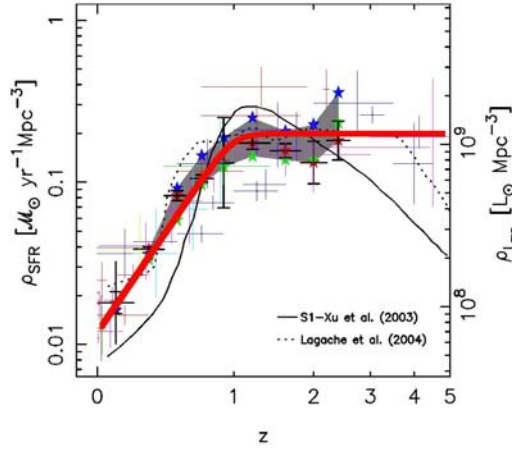
Fig. 1 The star formation rate as function of red-shift, compiled by Perez-Gonzalez et al. (2005). The colored points (shown with error bars) are extracted from different sources in the literature, normalized to the same standard cosmology. Red symbols are estimations based on H\alpha or H\beta measurements. Green symbols stand for [\text{OII}]\lambda 3737 estimations. UV-based data points are plotted in blue. Cyan estimations are based on mid-infrared data. The yellow point is based on X-ray data. The shaded area delimits the zone between two extreme SFR density estimations for each redshift. The horizontal bars show the range of redshifts used in each bin. The curves show two typical models: one with a decay from z = 1 , and another with a constant SFR density at high redshift. The thick (red) line is used in our calculations.
