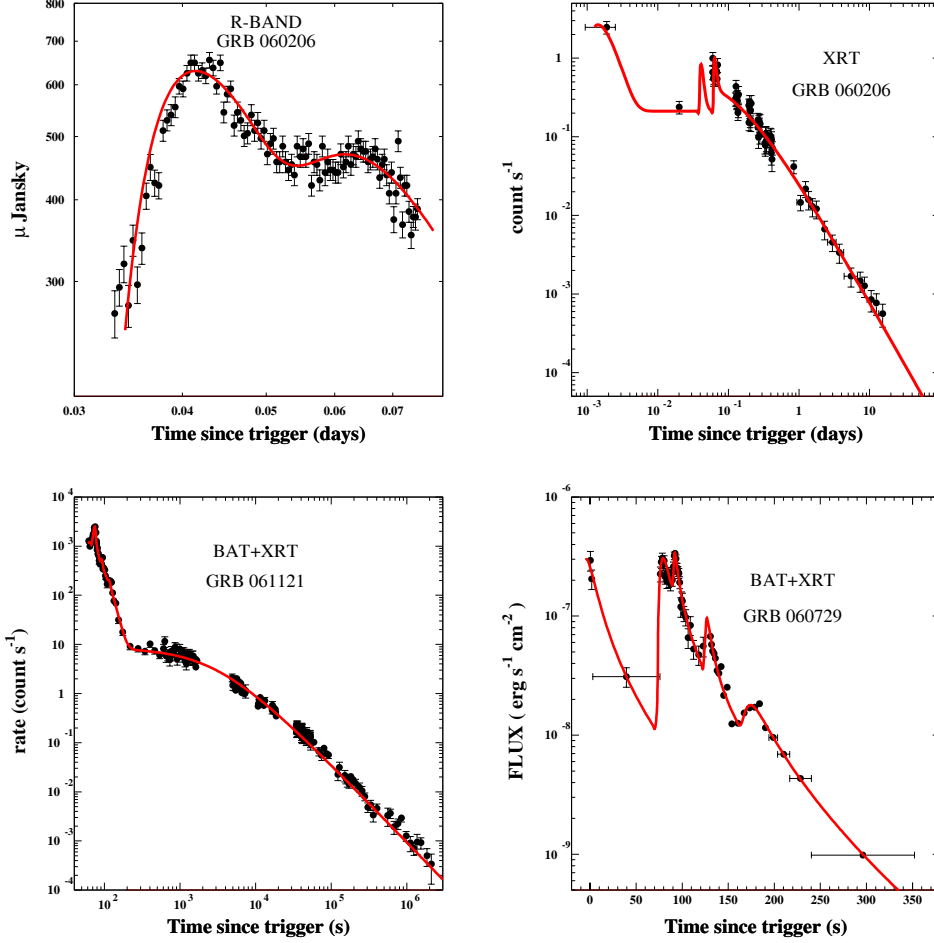
Fig. 5 (a) Top left : The very early R-band light curves of GRB 060206 (Wozniak et al. 2006). (b) Top right : The less-well sampled X-ray light curves (Evans et al. 2007), inferred from SWIFT BAT and XRT data for GRB 060206. The properties of the last two prominent X-ray flares are predicted from those of their optical counterparts in a. (c) Bottom left : The extensive X-ray light curve of GRB 061121 (Page et al. 2007). (d) Bottom right : The complex decay of the X-ray light curve of GRB 060729 (Grupe et al. 2007), with the progressively dying pangs of its accreting engine. All data are accompanied by their CB-model description (Dado et al. 2007c).
