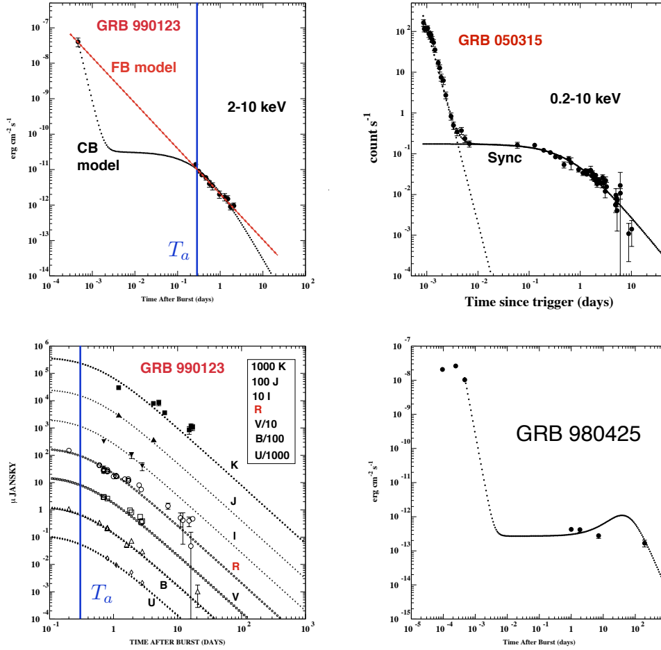
Fig. 1 (a) Top left: Pre-SWIFT predictions for the 2–10 keV X-ray AG in the CB (DDD02) and fireball (e.g. Maiorano et al. 2005) models, compared to data for GRB 990123. T_a is the time ending the ‘plateau’ phase. (b) Top right: Comparison between the CB model prediction and the canonical 0.2–10 keV X-ray light curve of GRB 050315 (Vaughan et al. 2006). (c) Bottom left: Broad band optical data on GRB 990123, fit in the CB model (DDD03). After the onset of the plateau, the predicted and observed evolution is achromatic from optical to X-ray energies, as seen in this figure and its comparison with (a). (d) Bottom right: The X-ray light curve of GRB 980425 (DDD02) showing a ‘canonical’ behaviour and what we called a ‘plateau’ (long and hilly in this case, given the large observer’s angle). The last (red) point postdates the original figure. The other properties of this GRB and its SN are also not exceptional, in the CB model (DDD03).
