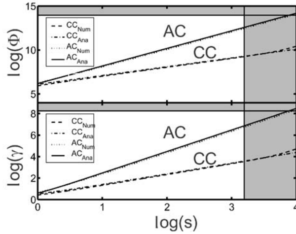
Fig. 2 Accelerated potential drop ( \Phi ) and Lorentz factor ( \gamma ) as functions of distance s from stellar surface in the AC and CC for an aligned anti-parallel rotator, s is in units of cm and \Phi is in units of Volt. “AC” and “CC” denote “annular cap” and “core cap”, subscripts ‘Num’ and ‘Ana’ refer to numerical solution and analytic approximation. The shaded area mark the regions where the 1-D annular polar cap acceleration solution is no longer valid. The parameters used here are the usual values for \gamma -ray pulsar (i.e. p = 0.1 s, B = 10^{12} G).
