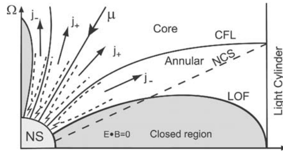
Fig. 1 A schematic diagram for the annular and the core regions for an inclined rotator, \Omega and \mu are the rotational and magnetic axis, respectively. The null change surface (NCS) is the surface where the magnetic field is perpendicular to the rotation axis (i.e. \Omega \cdot \mathbf{B} = 0 ). Line ‘CFL’ and ‘LOF’ are the critical field line and the “last” open field line, respectively. Charged particles with opposite signs leave off the annular and the core cap regions, respectively. The upper boundaries of the pair formation front are denoted by the dashed lines. The “flash” symbols indicate the locations with the maximal possibility to initiate the pair-production cascade.
